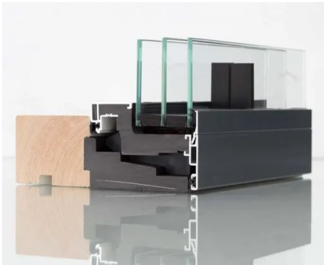
Windows Triple glazed aluminium/ timber composite
