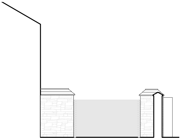
Proposed gate opening Repairs to existing piers New freestanding 2m high timber slatted fence
