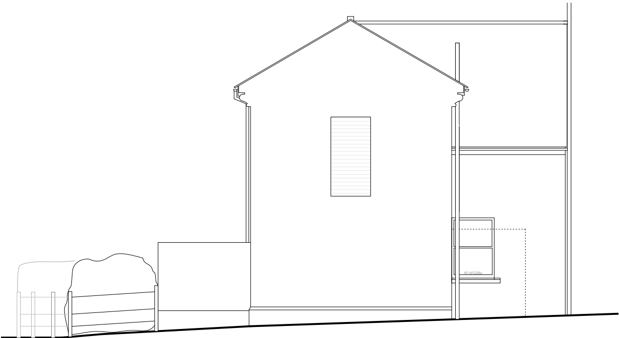
South Elevation
