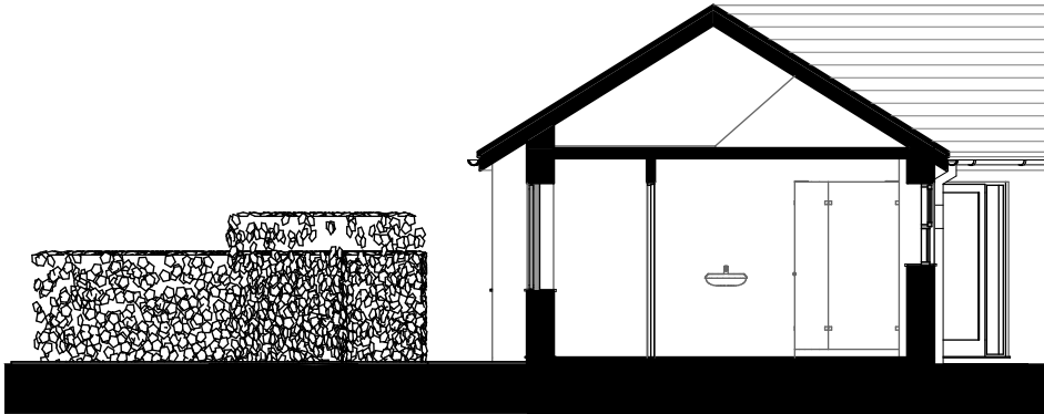
S-01 Building Section 1:100
