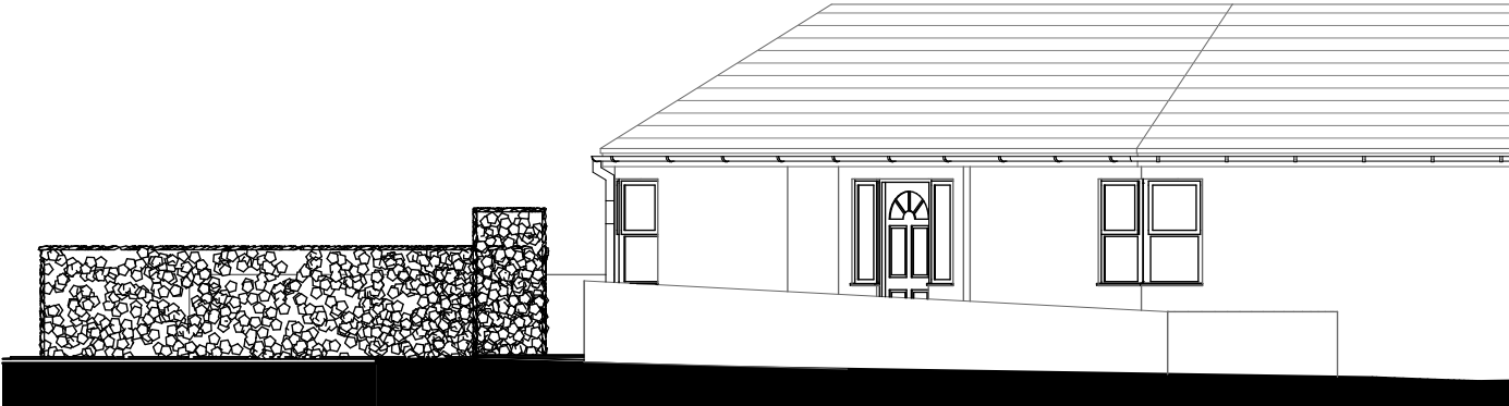
E-01 Southeast Elevation 1:100
