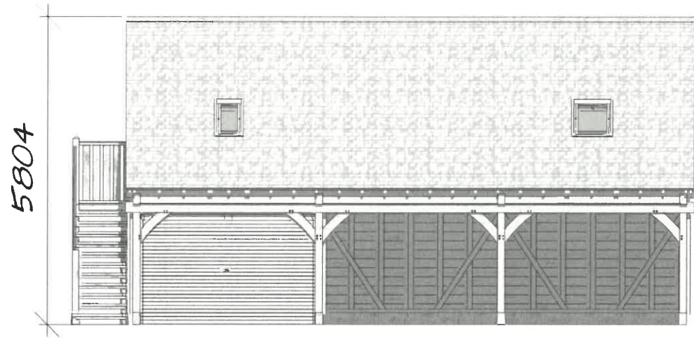
PROPOSED WEST ELEVATION
