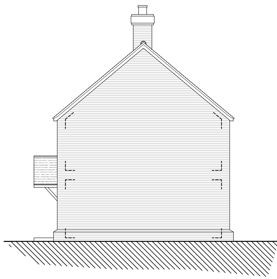
WEST ELEVATION
