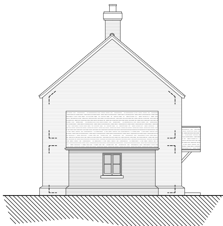
EAST ELEVATION
