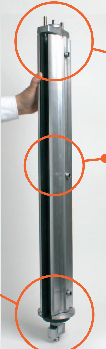
Demountable Post MG_4510/4 Delivered as complete units directly from the factory. They should only be disassembled for general maintenance purposes and seal replacement when necessary.
