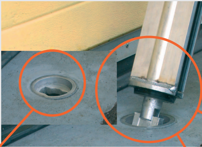
Ground Insert Dust Caps MG_4520/4
