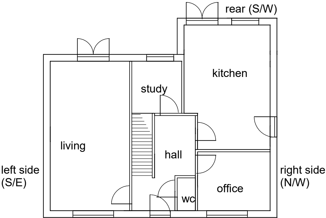
front (N/E) GROUND FLOOR LAYOUT
