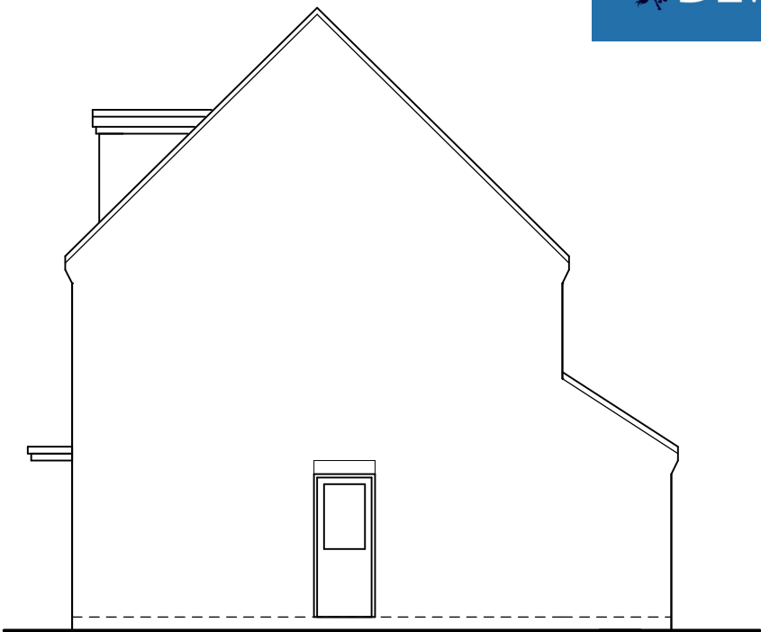
right side (northwest) elevation
