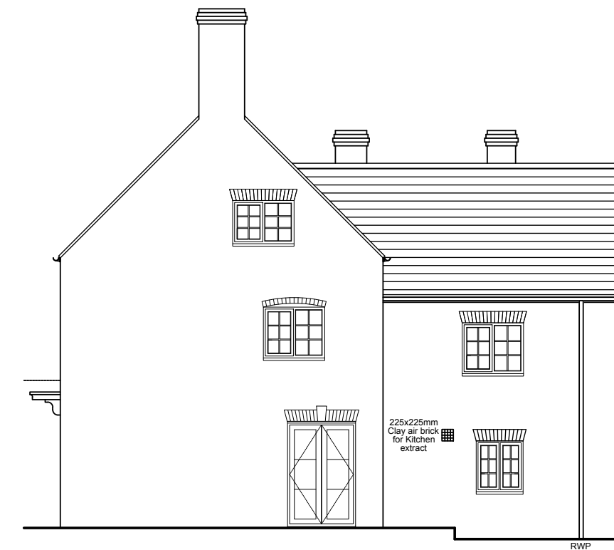
EXISTING EAST FACING ELEVATION Scales 1:100 @ A2
