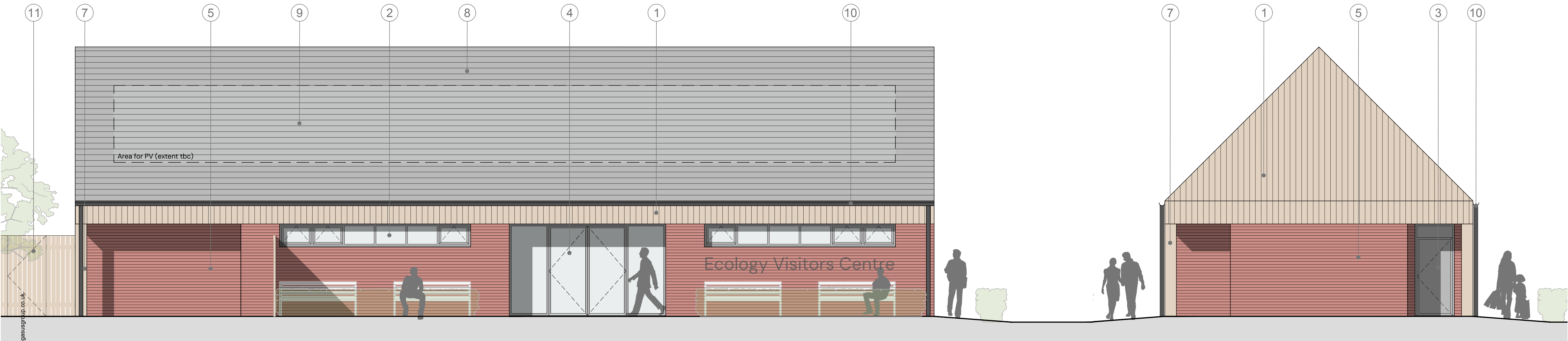
Front Elevation (facing the carpark)
