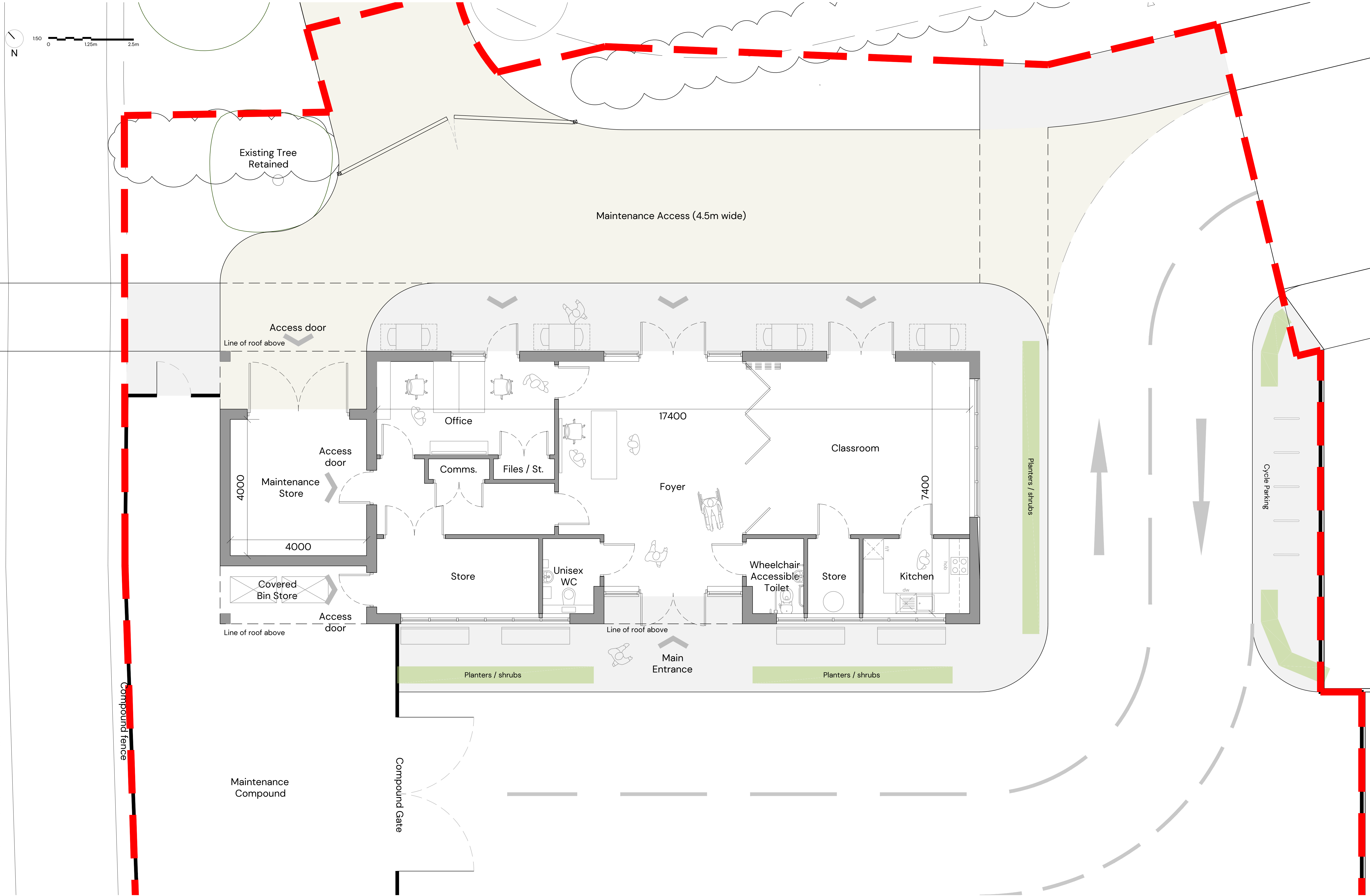
Proposed Ground Floor Plan - Ashton Park, Ecology Visitors Centre
