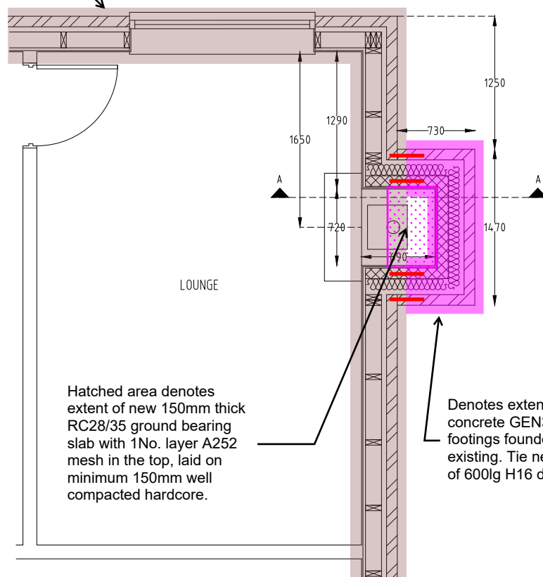
FOUNDATION PLAN
