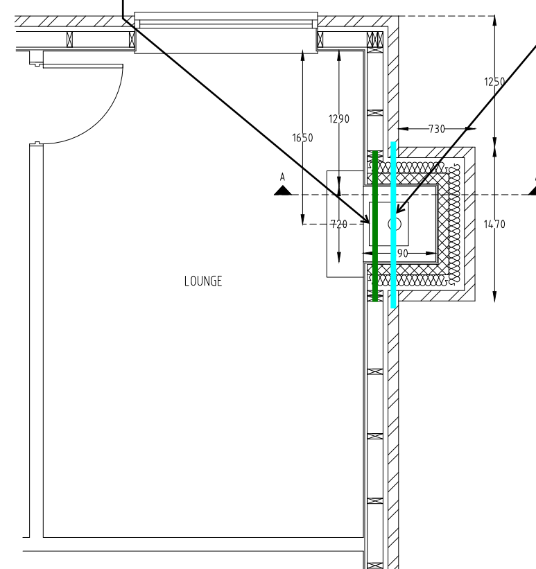
SUPERSTRUCTURE PLAN
