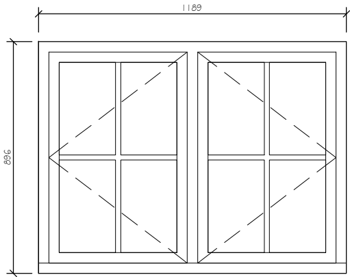
Window No. WGO7 Timber framed double glazed casement with stone cill to match existing in existing opening
