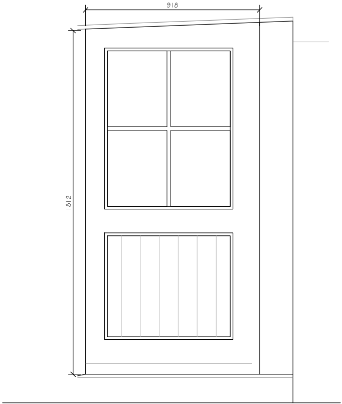
Window No. WGO4 Timber framed double glazed window/door in existing opening
