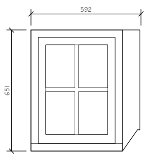
Window No. WGO8 Timber framed double glazed fixed casement with stone cill to match existing
