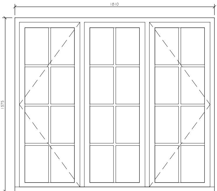
Window No. WGO5 Timber framed double glazed casement with stone cill to match existing in modified existing opening
