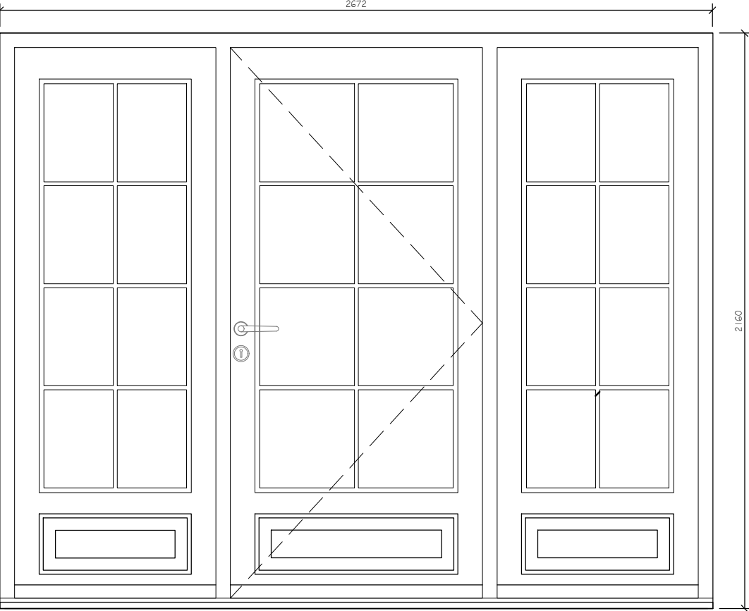
Window No. WFO3, WFO4 Timber framed double glazed casement to refurbished existing dormer
