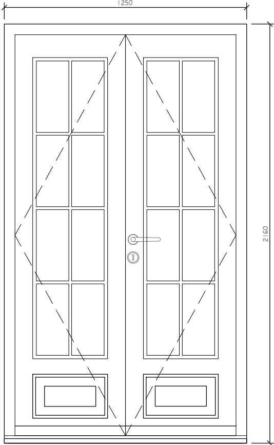
Door No. DG03 Timber framed double glazed French doors to existing opening
