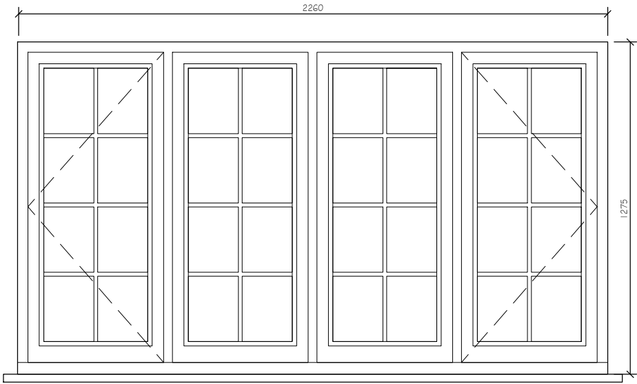
Window No. WGO1 Timber framed double glazed casement with stone cill to match existing in existing opening
