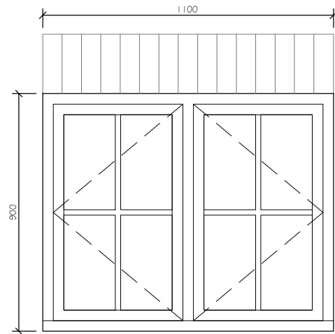
Window No. WGO6 Timber framed double glazed casement with stone cill to match existing in existing opening
