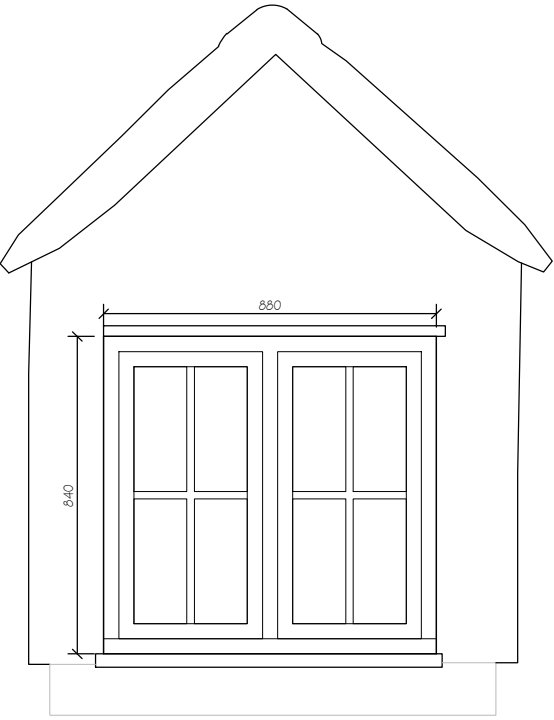
Window No. WGO2, WGO3 Timber framed double glazed casement with stone cill to match existing in existing opening
