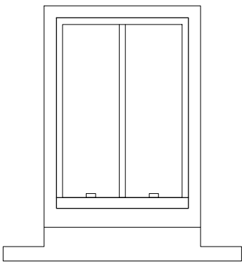
Roof light, RLO1, RLO2 Replacement conservation rooflights to existing opening
