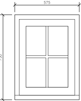
Window No. WFO5 Timber framed double glazed casement in existing opening
