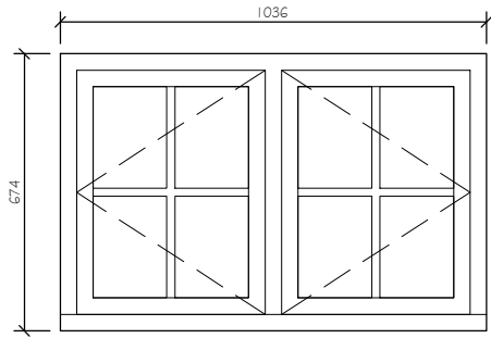
Window No. WFO1, WFO2 Timber framed double glazed casement to existing opening
