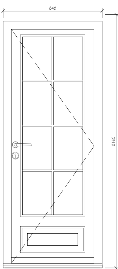
Door No. DG04 Timber framed double glazed French door to existing opening
