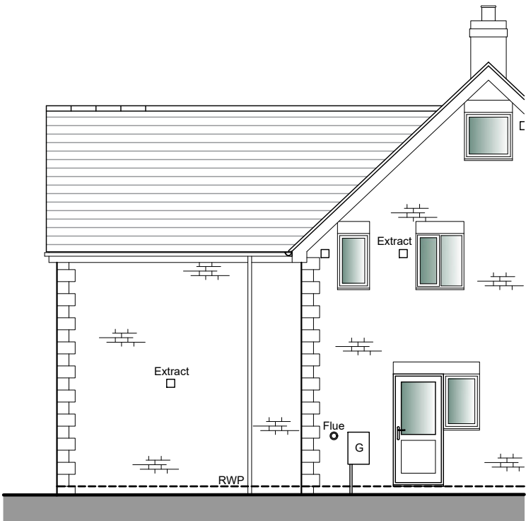
Part North East Elevation
