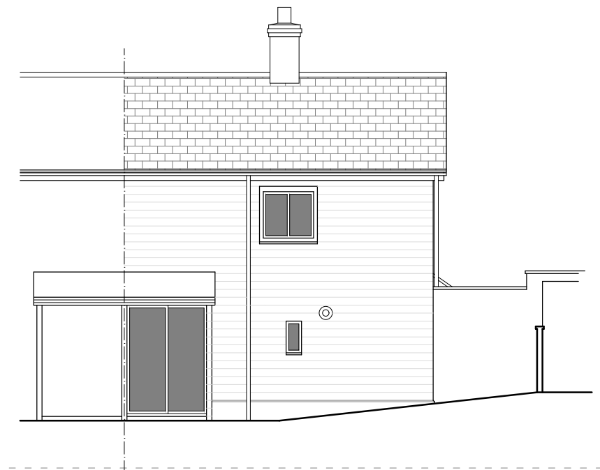
FRONT (NORTH) ELEVATION - scale 1:100
