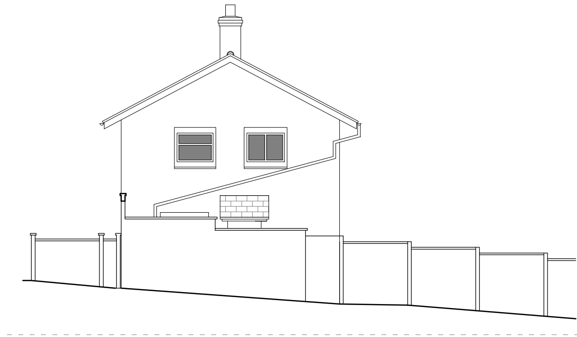
SIDE - LANE (WEST) ELEVATION - scale 1:100
