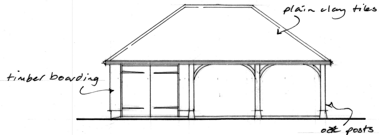
EAST ELEVATION
