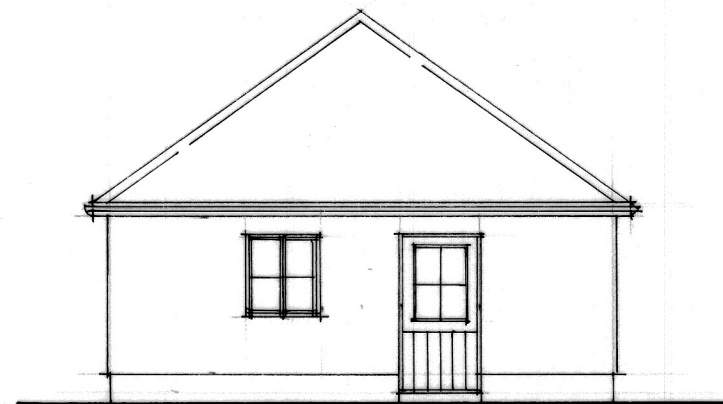
NORTH ELEVATION
