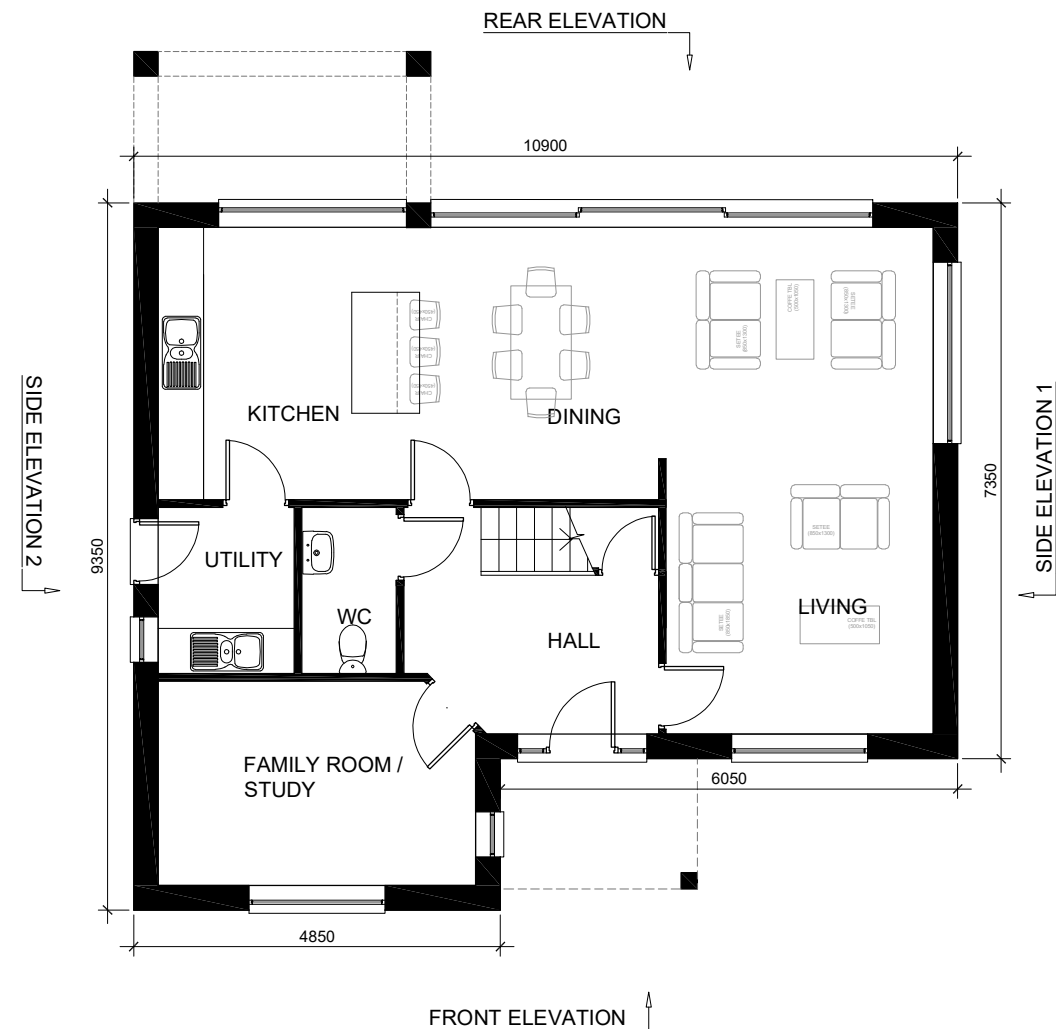
GROUND FLOOR PLAN AS PROPOSED GIA - 77m²
