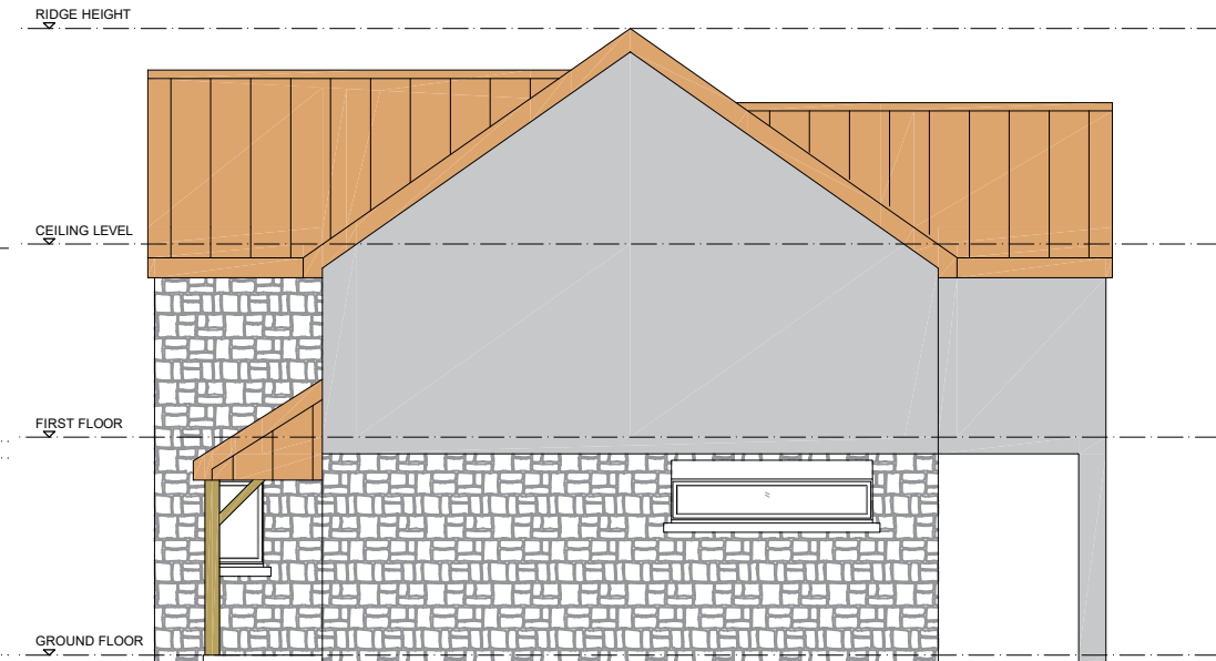
SIDE ELEVATION 1 AS PROPOSED
