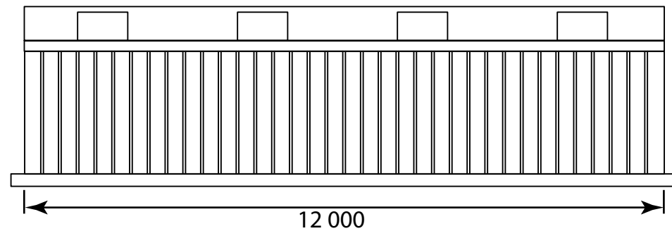
East Elevation (1:100)
