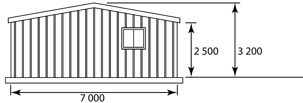
North Elevation (1:100)
