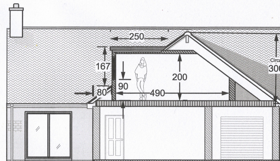
North East Elevation proposed- section A -A
