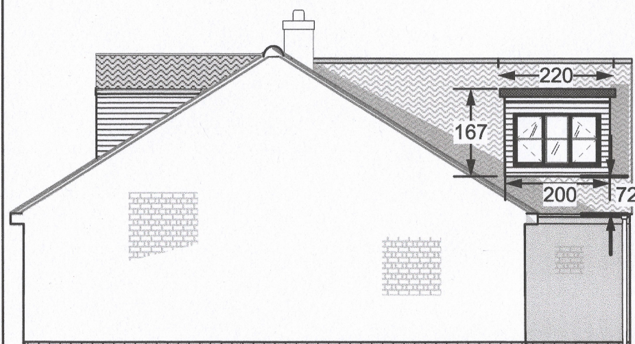
South East Elevation Proposed
