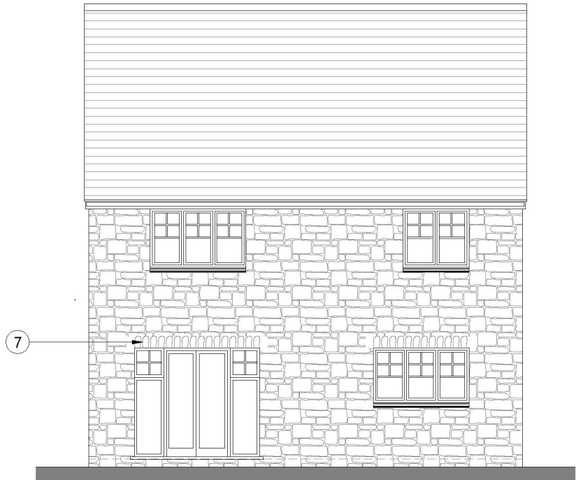
Rear Elevation
