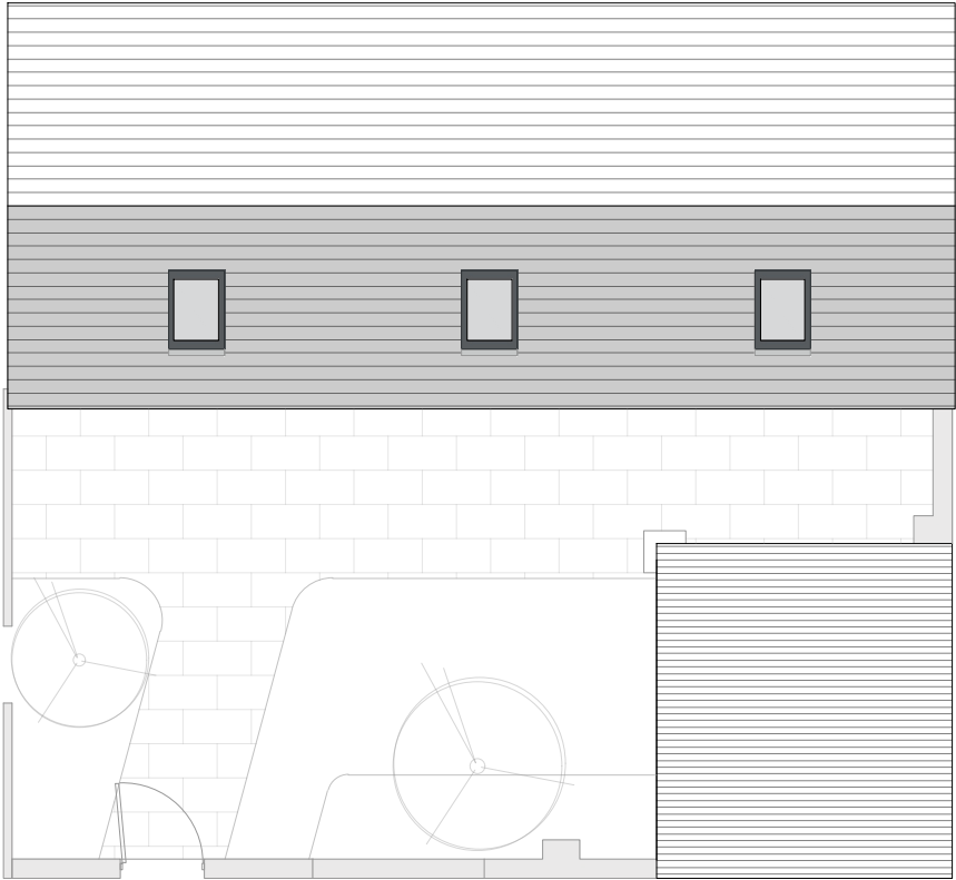
West Elevation - As Proposed
