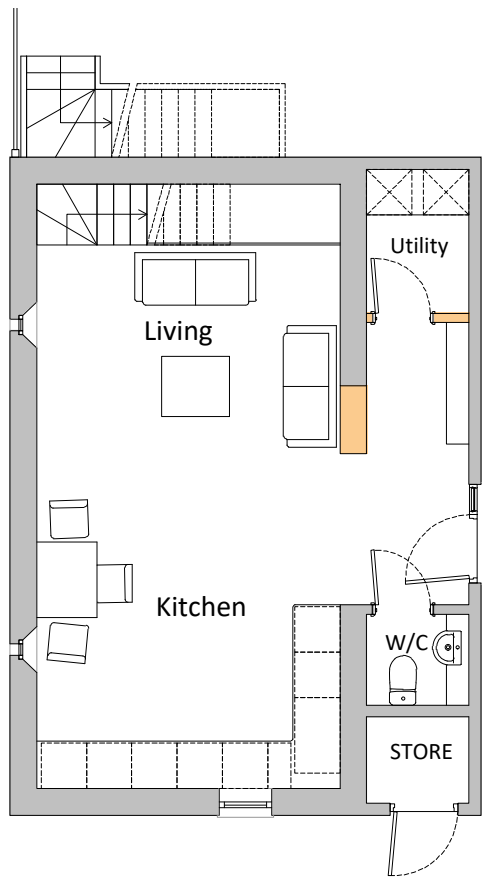
Ground Floor Plan - As Proposed
