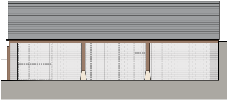
West Elevation - As Existing
