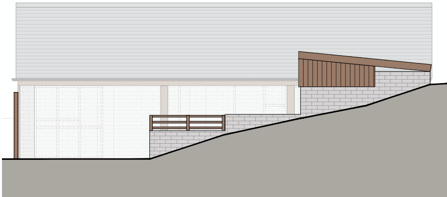
West Elevation - As Existing
