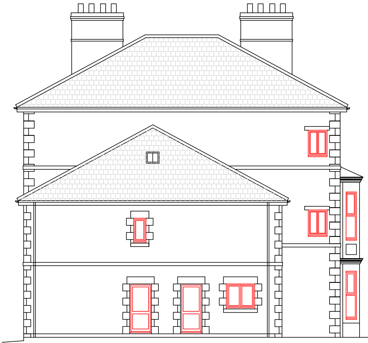
Proposed Side (West) Elevation 1:100
