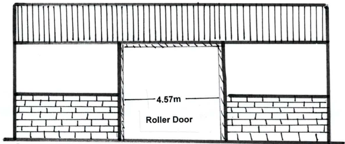
Southern Elevation
