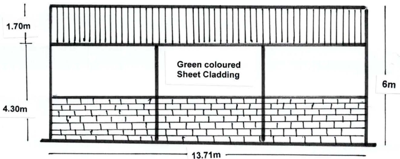
Northern Elevation
