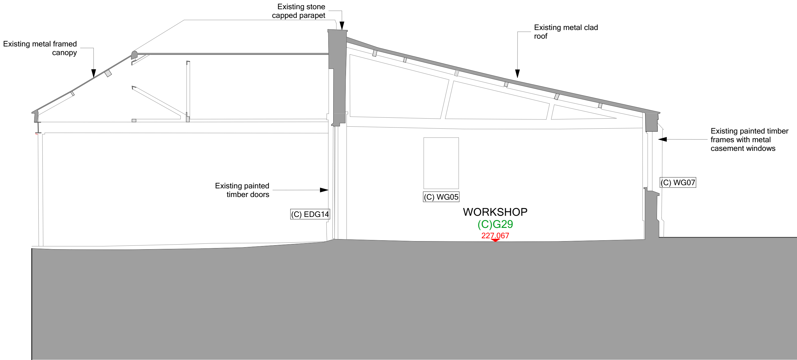
SECTION 8-8
