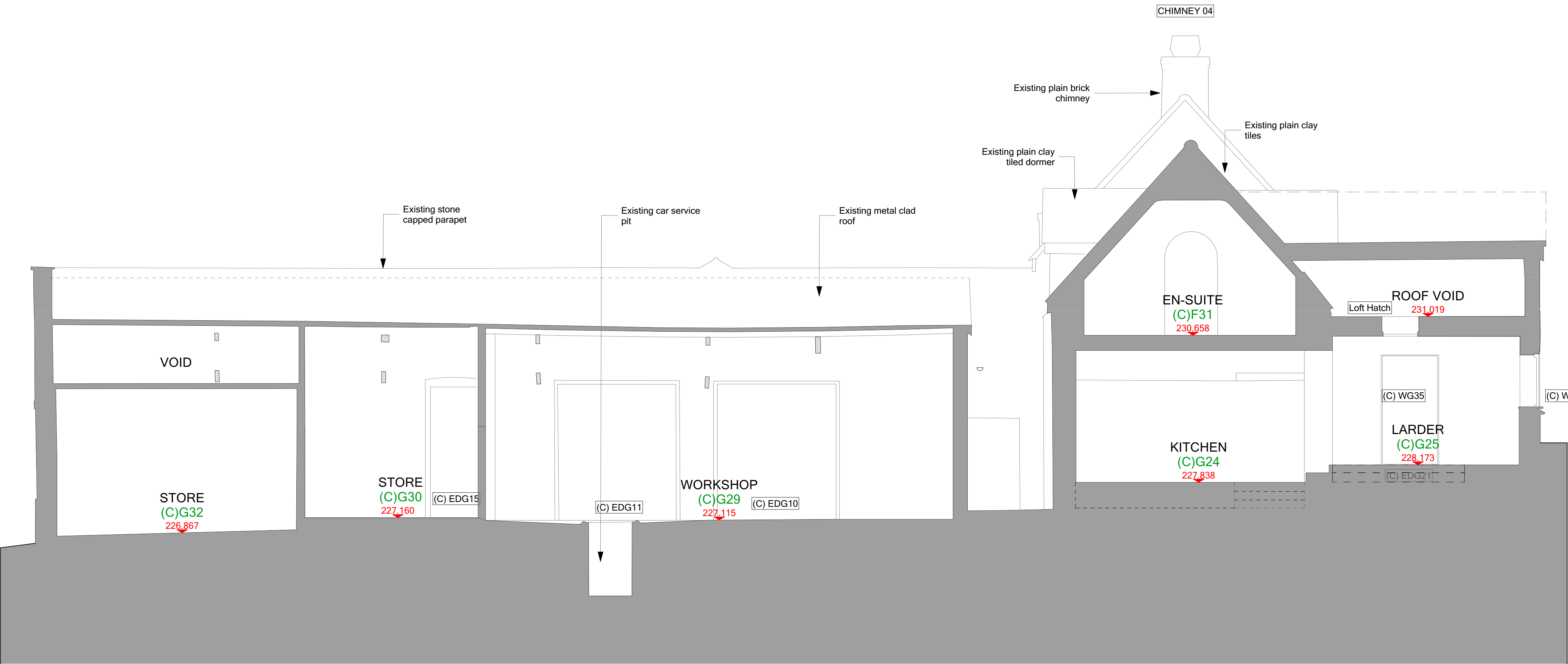
SECTION 7-7
