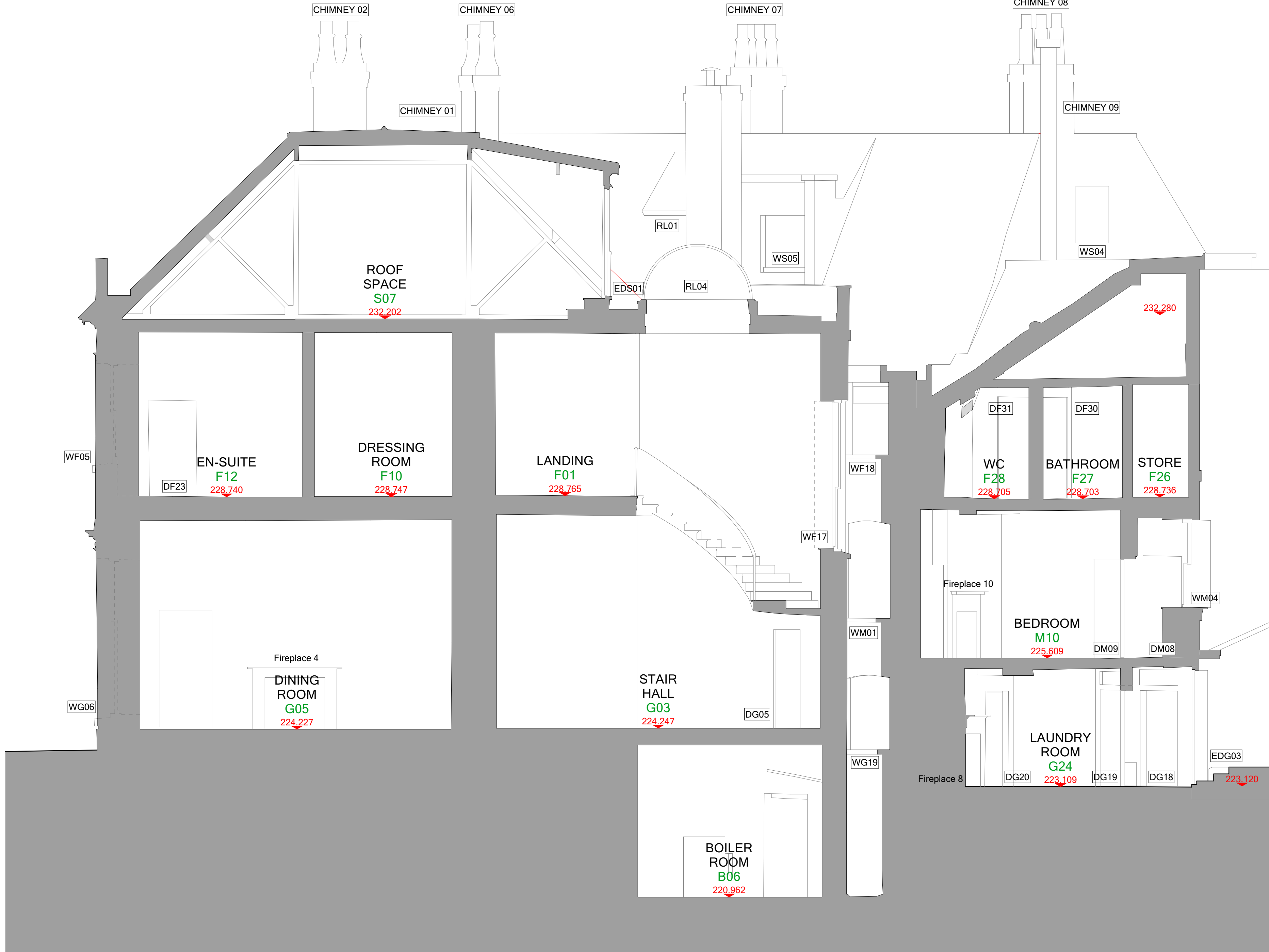
SECTION F-F
