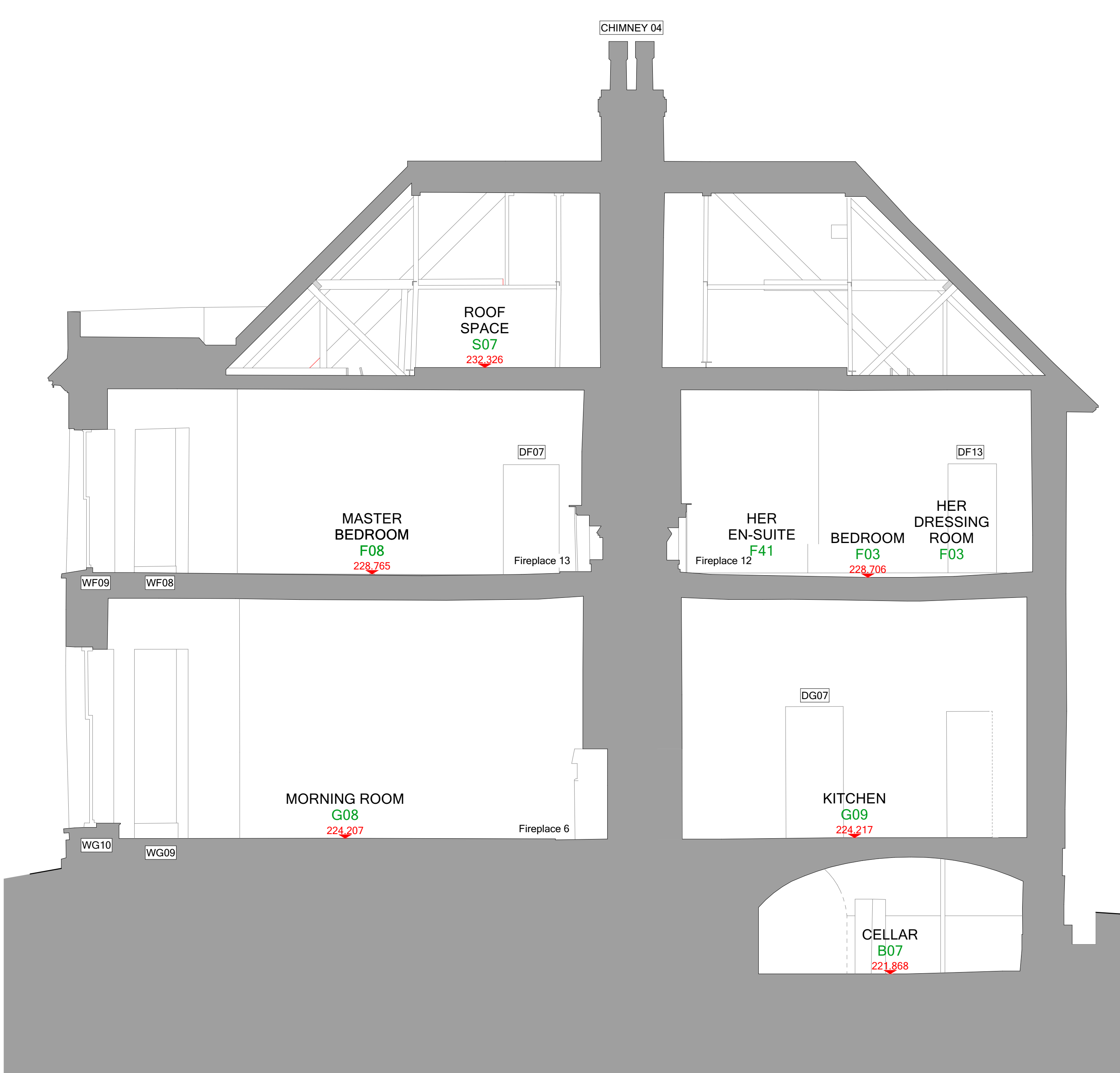
SECTION E-E
