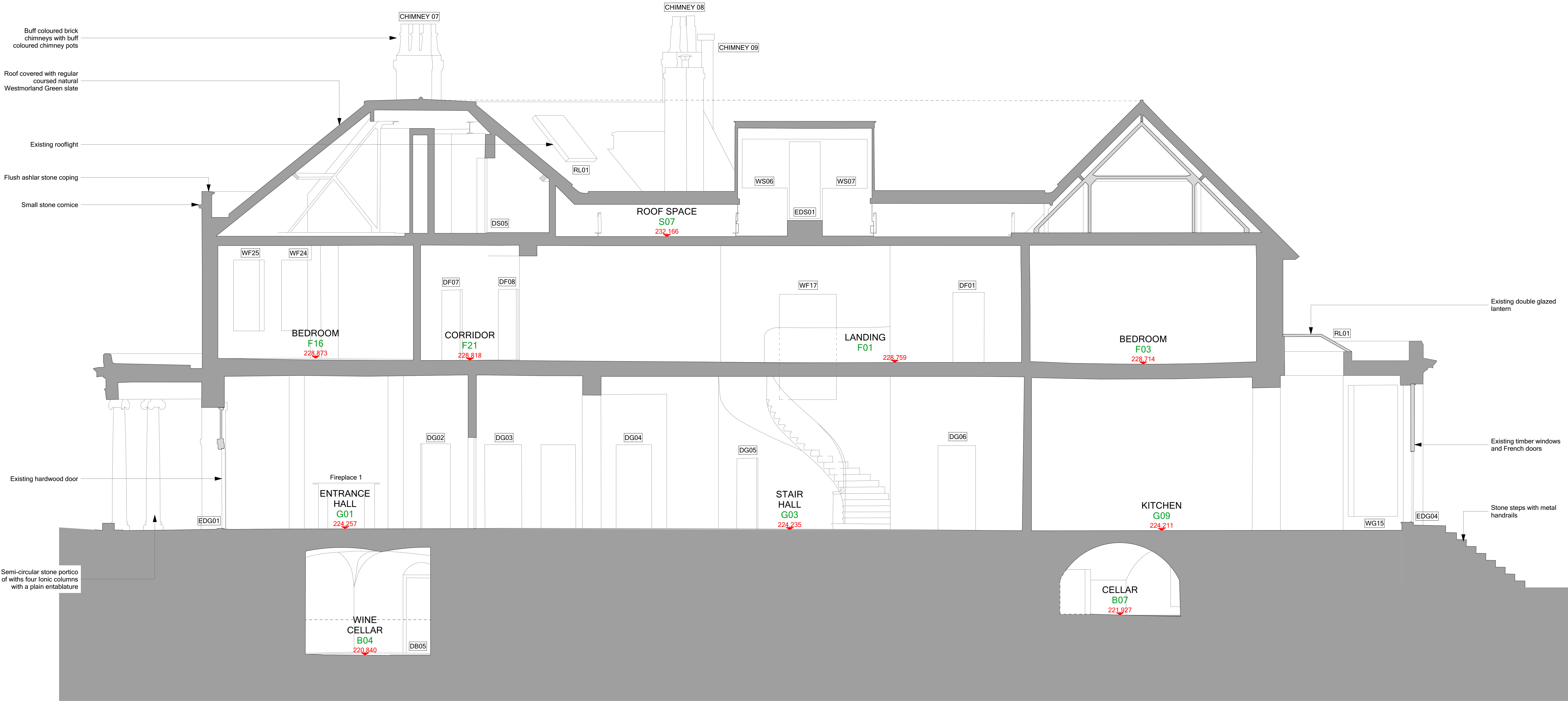
SECTION B-B
