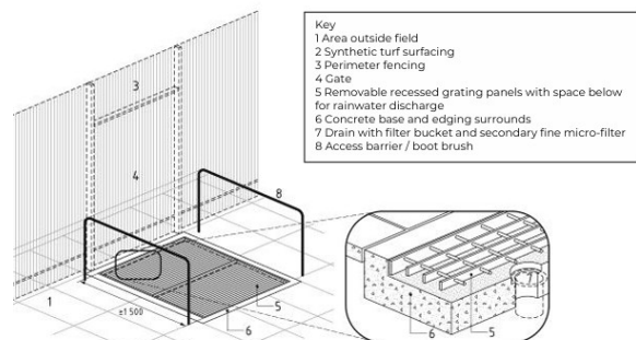
Example Detox grate outside a 3G pitch
