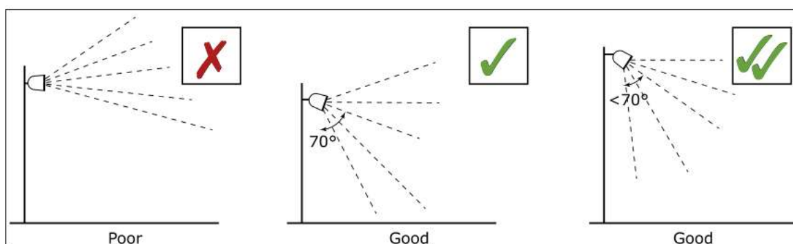
Figure 5 – Light angle tilt to not contribute to sky glow
