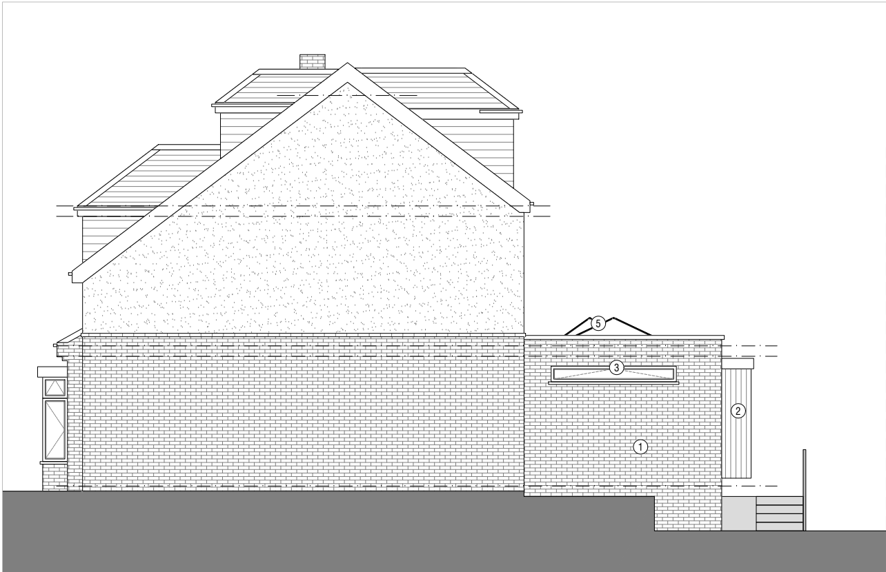
04 - Side Elevation (South-West)
