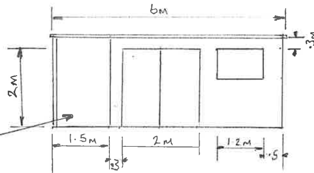
SIDE ELEVATION
