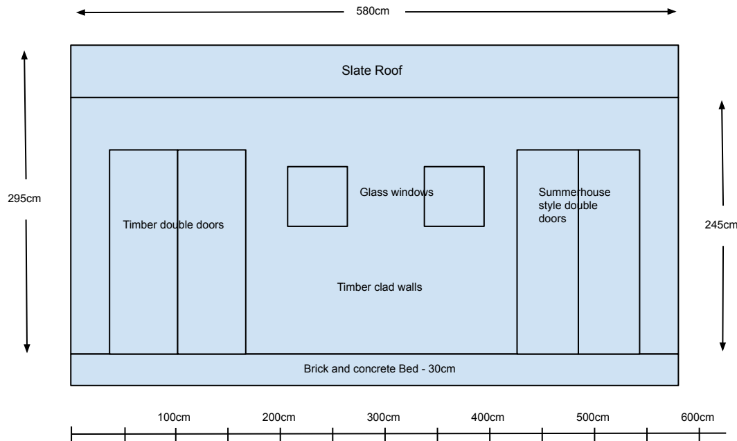
Shed Side - 1:50 scale
