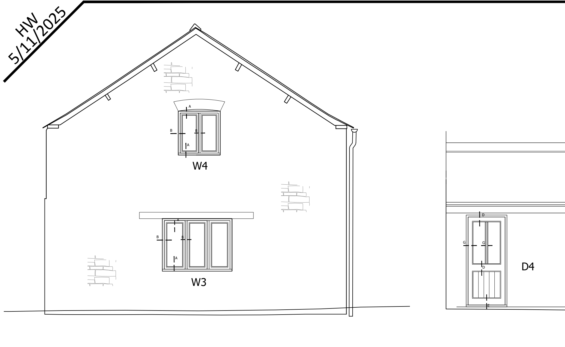
West elevation
