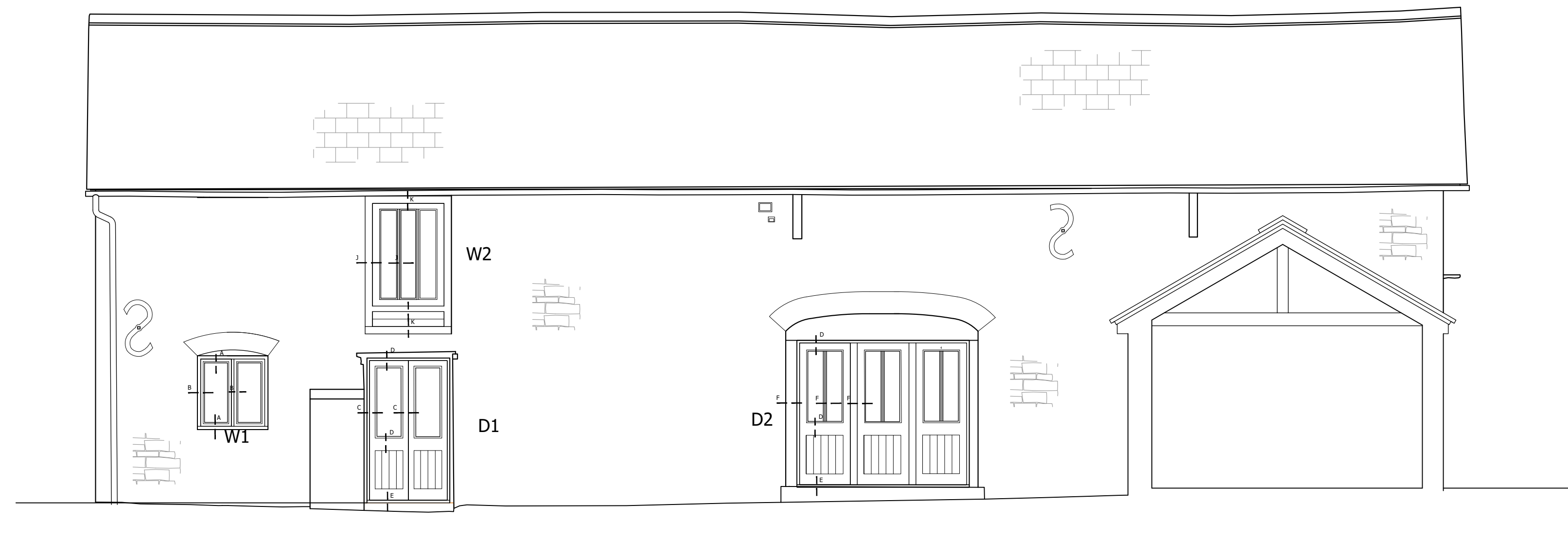
South elevation
