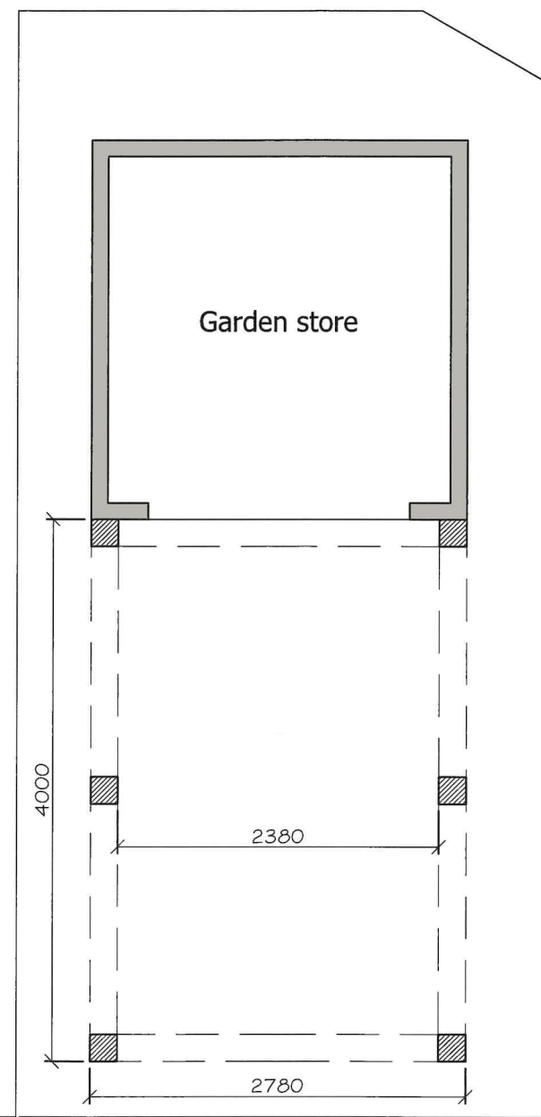
Proposed Plan
