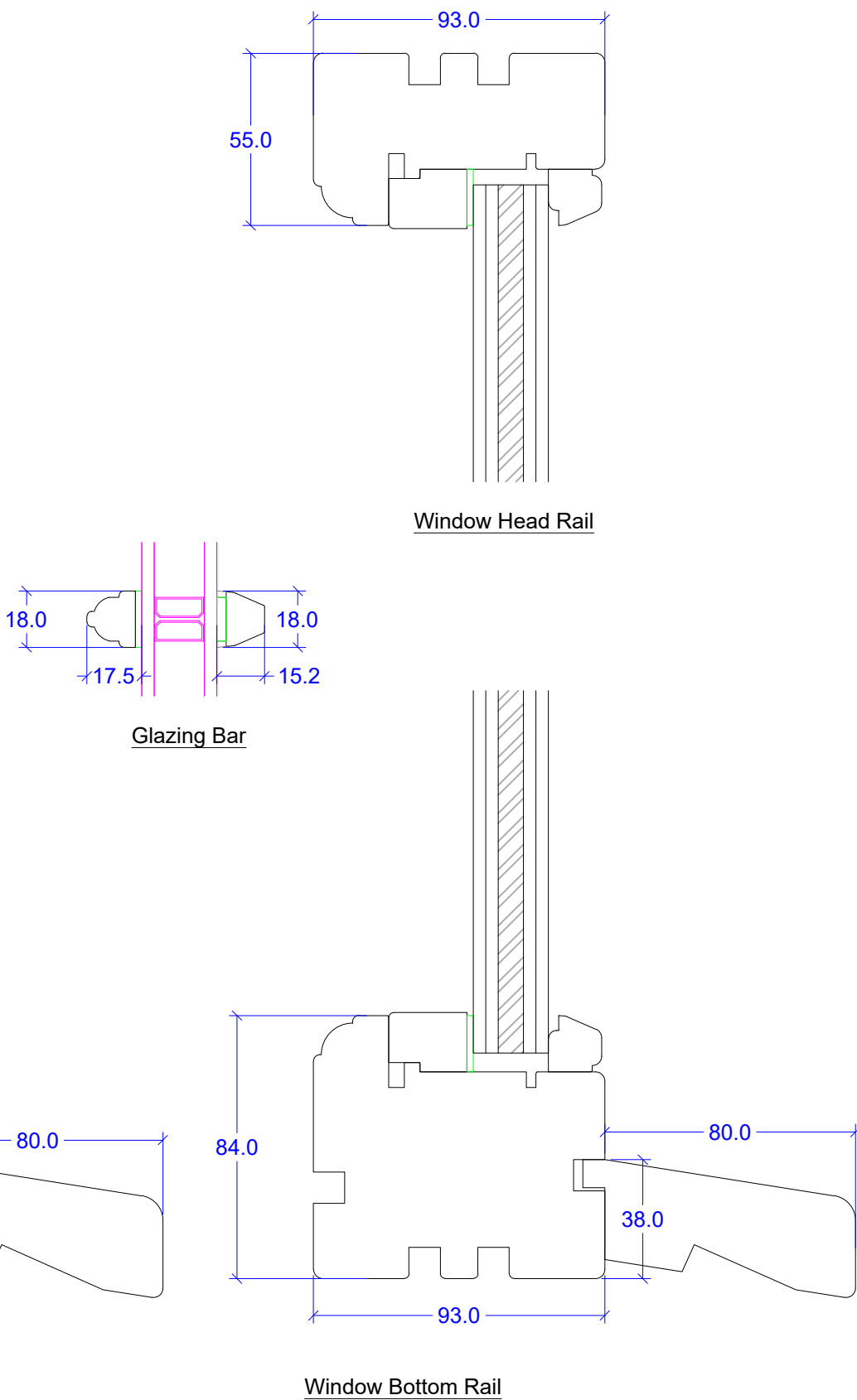
VERTICAL VIEW THROUGH PANELLED FRAME
