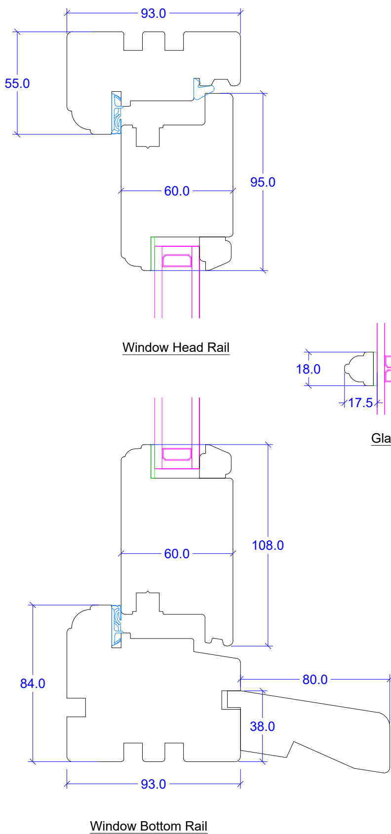
VERTICAL VIEW THROUGH WINDOW
