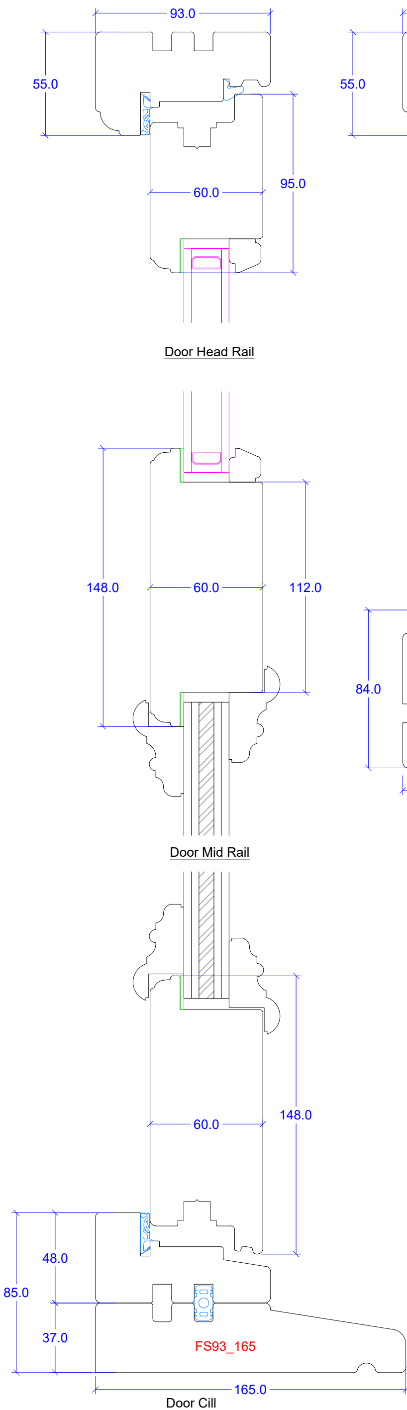
VERTICAL VIEW THROUGH DOUBLE DOOR
