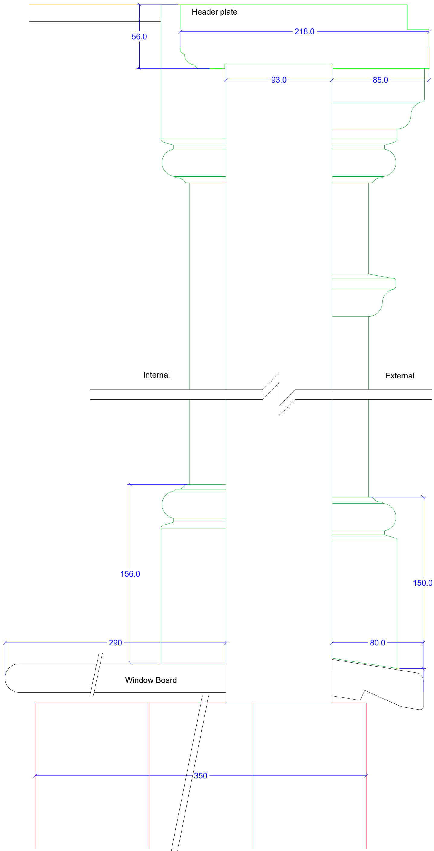
VERTICAL VIEW THROUGH PILASTER
