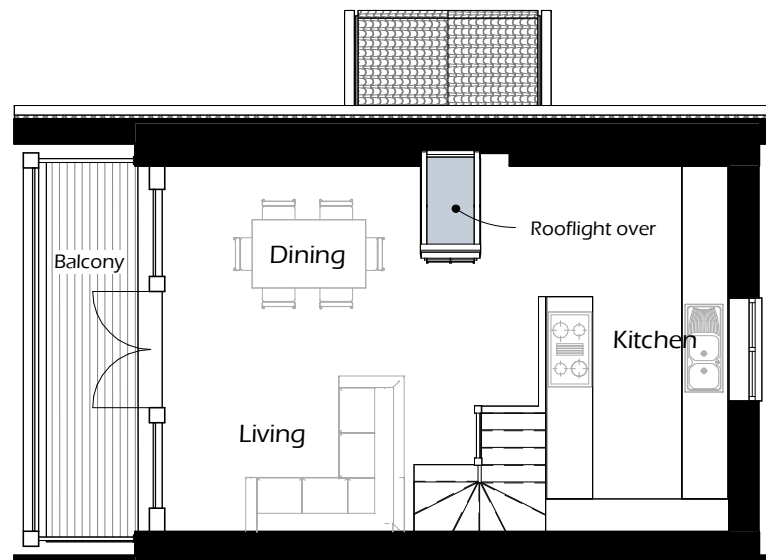
2 First Floor Plan 1 : 100
