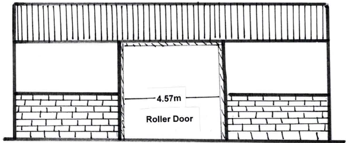
Southern Elevation
