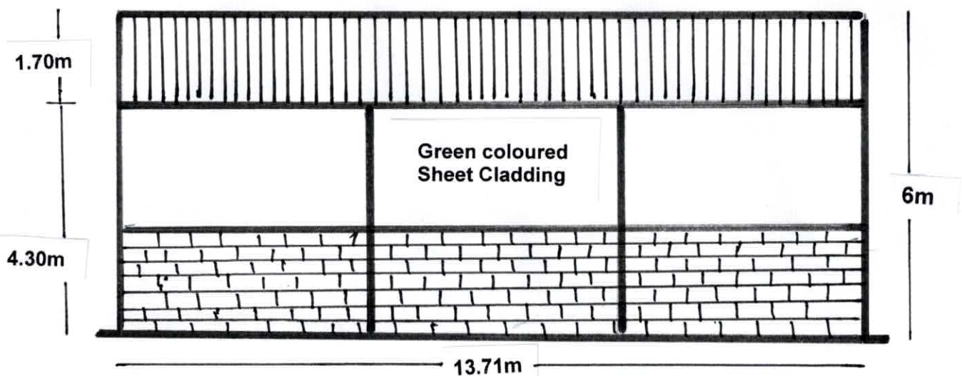
Northern Elevation
