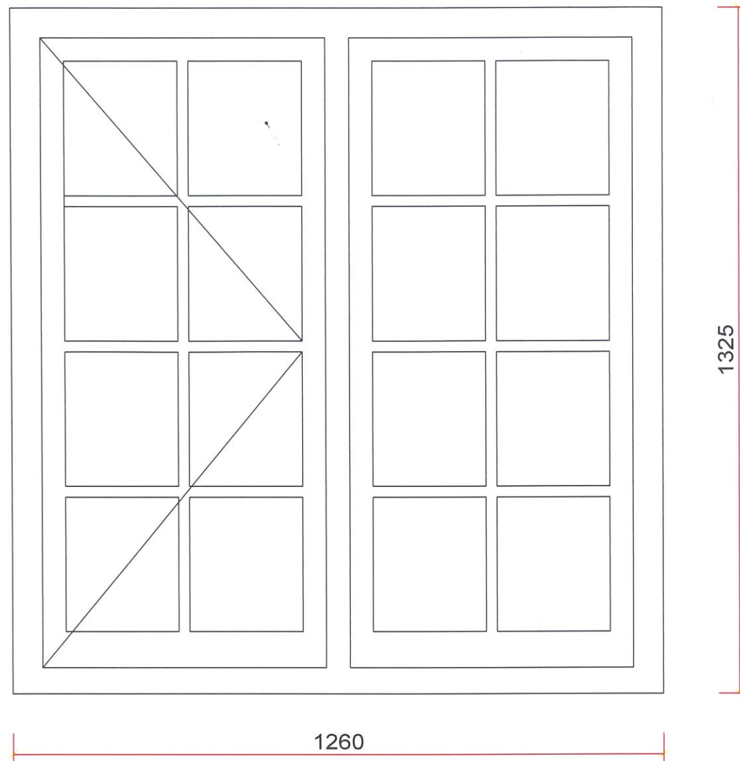
W3 Dormer Window
