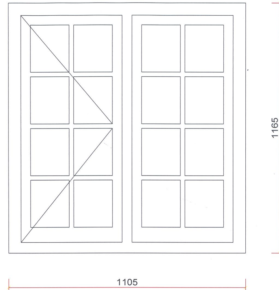
W2 1st Floor
