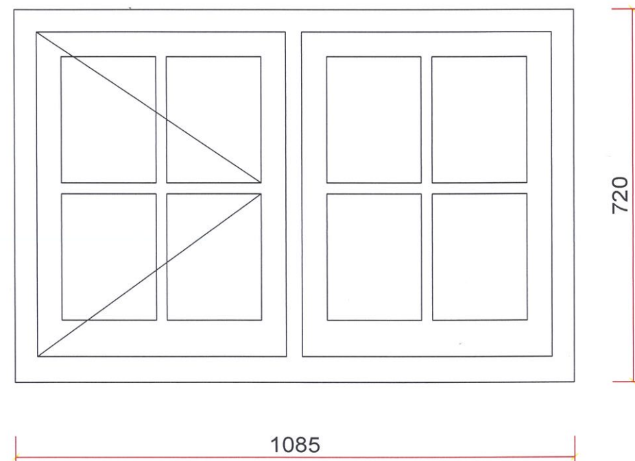
W3 Dormer Window
