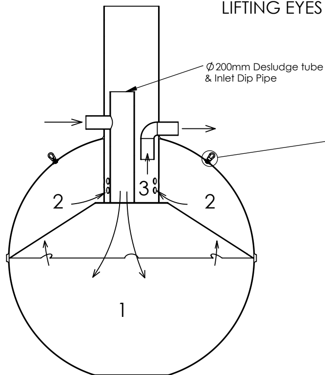
SECTION VIEW
