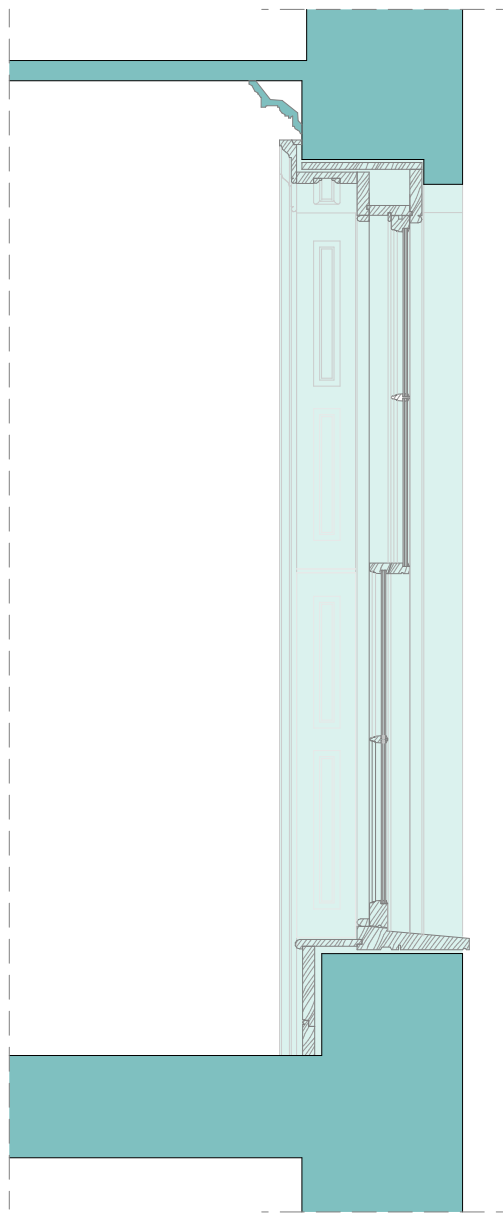
Section S1 Timber sash window with linear head
