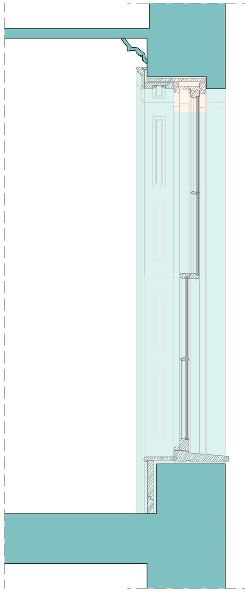
Section S2 Timber segmental arch sash window. Brick opening and structural opening remain unaltered while the top section of the joinery is proposed as arched.
