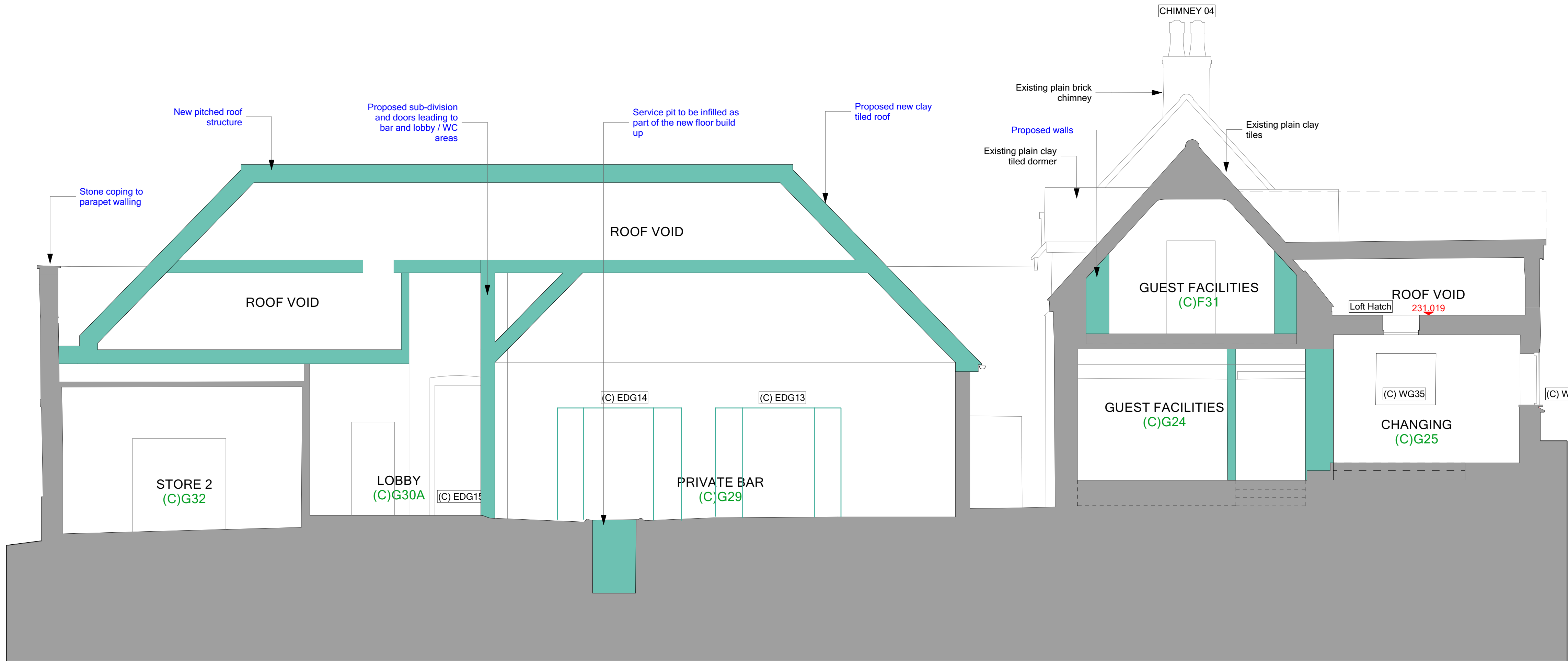
SECTION 7-7
