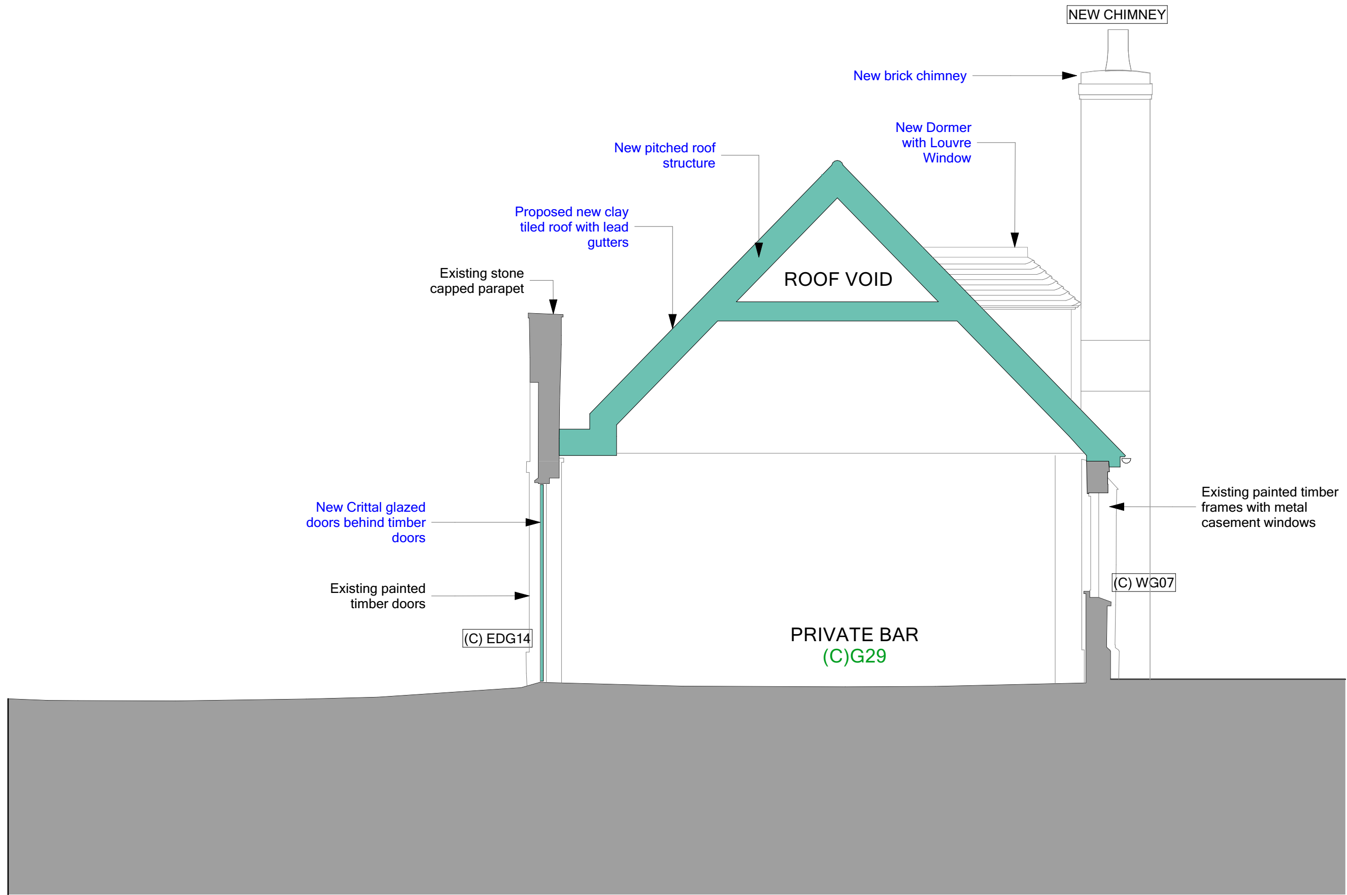
SECTION 8-8
