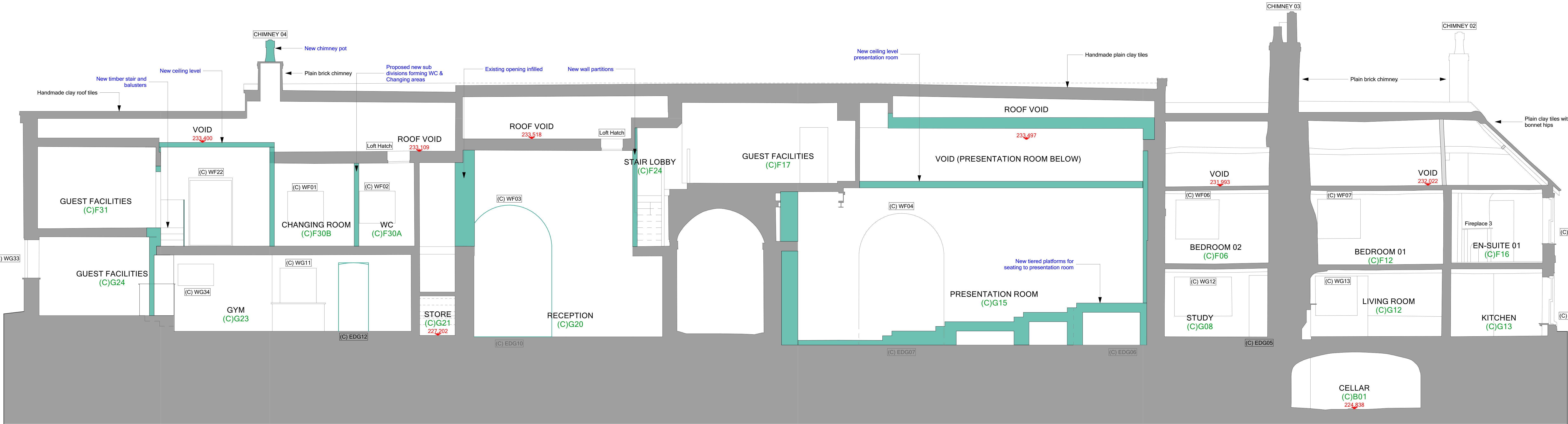
SECTION 6-6
