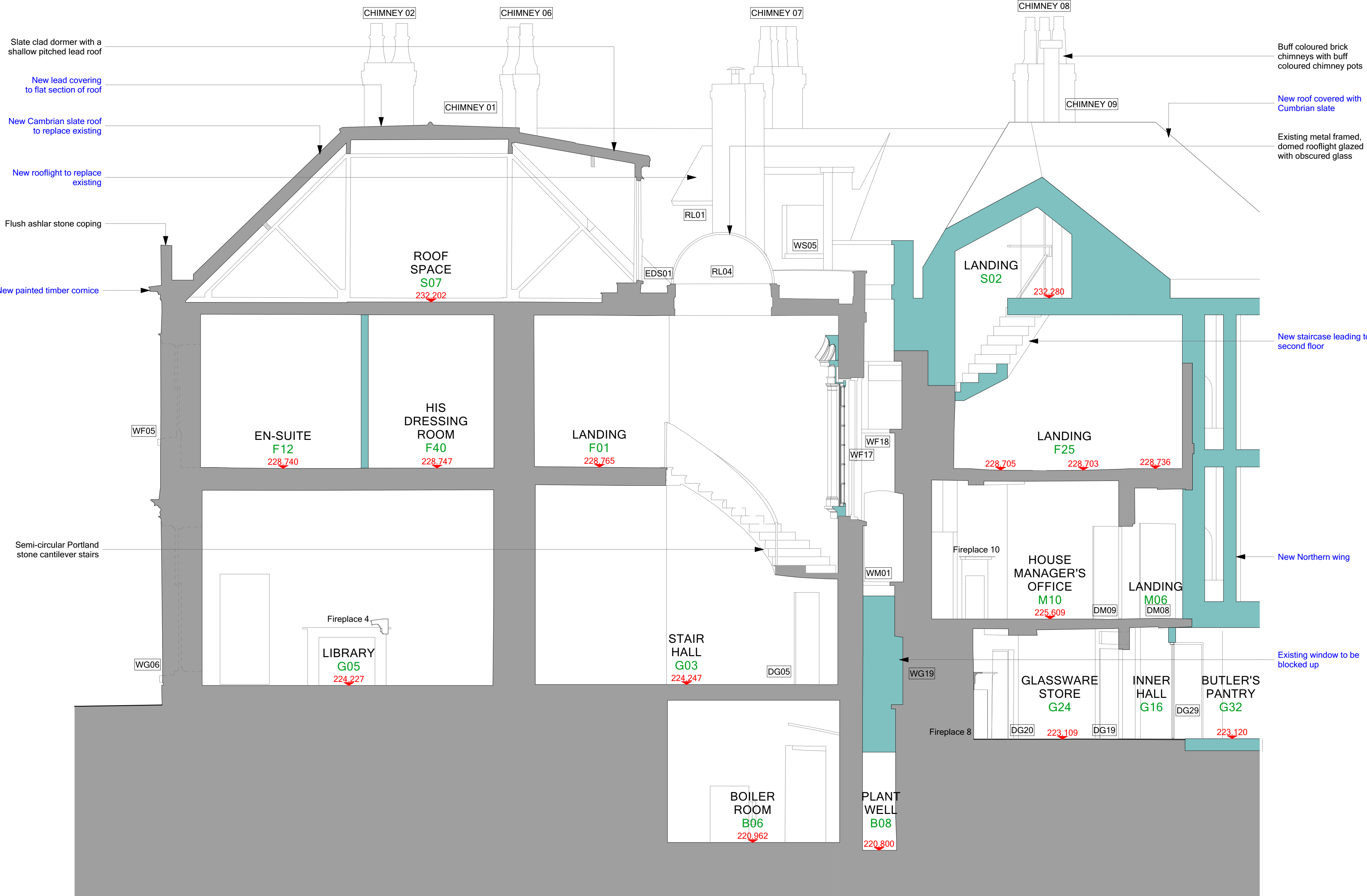
SECTION F-F
