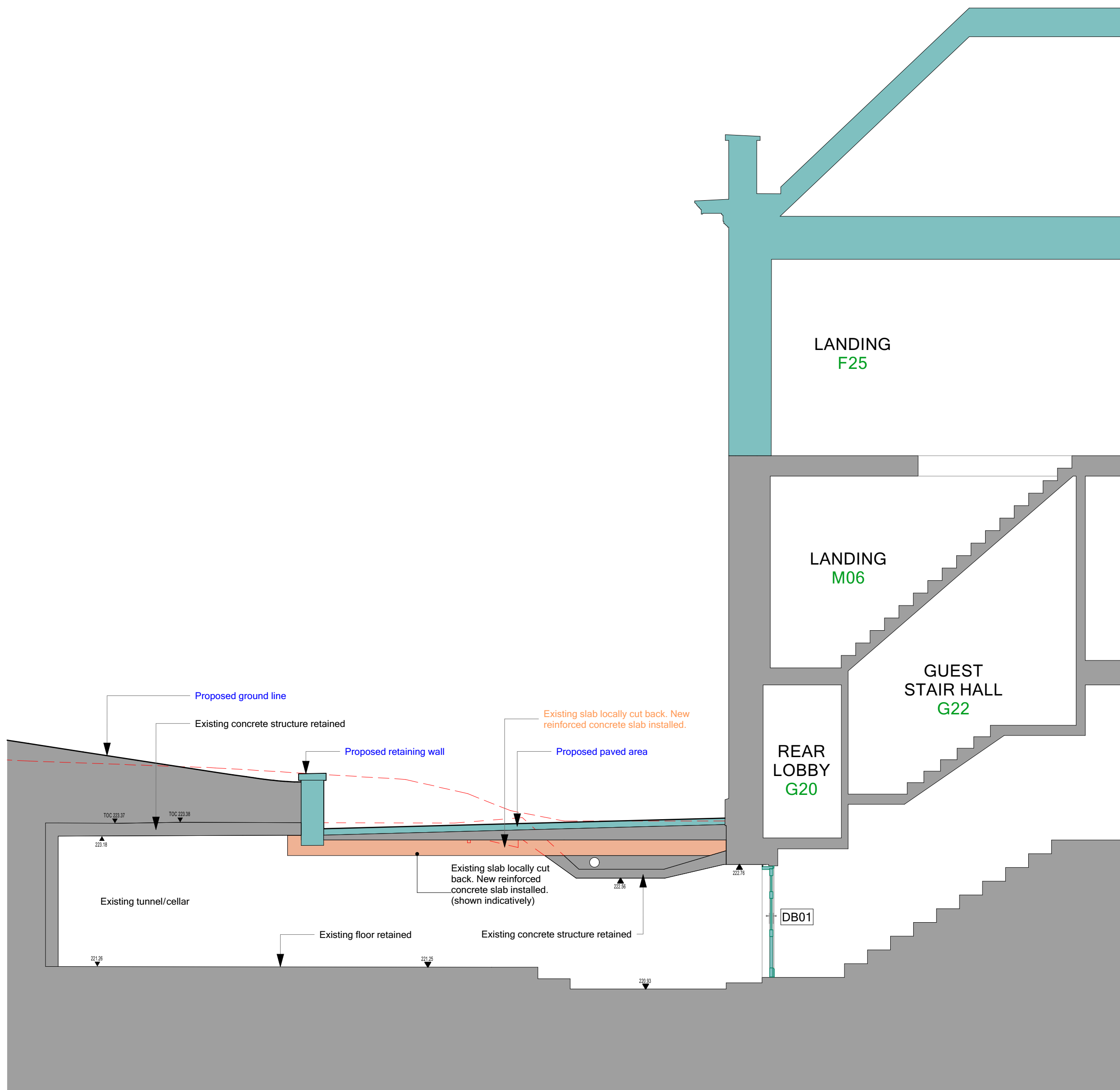
SECTION H-H - ARP Tunnel
