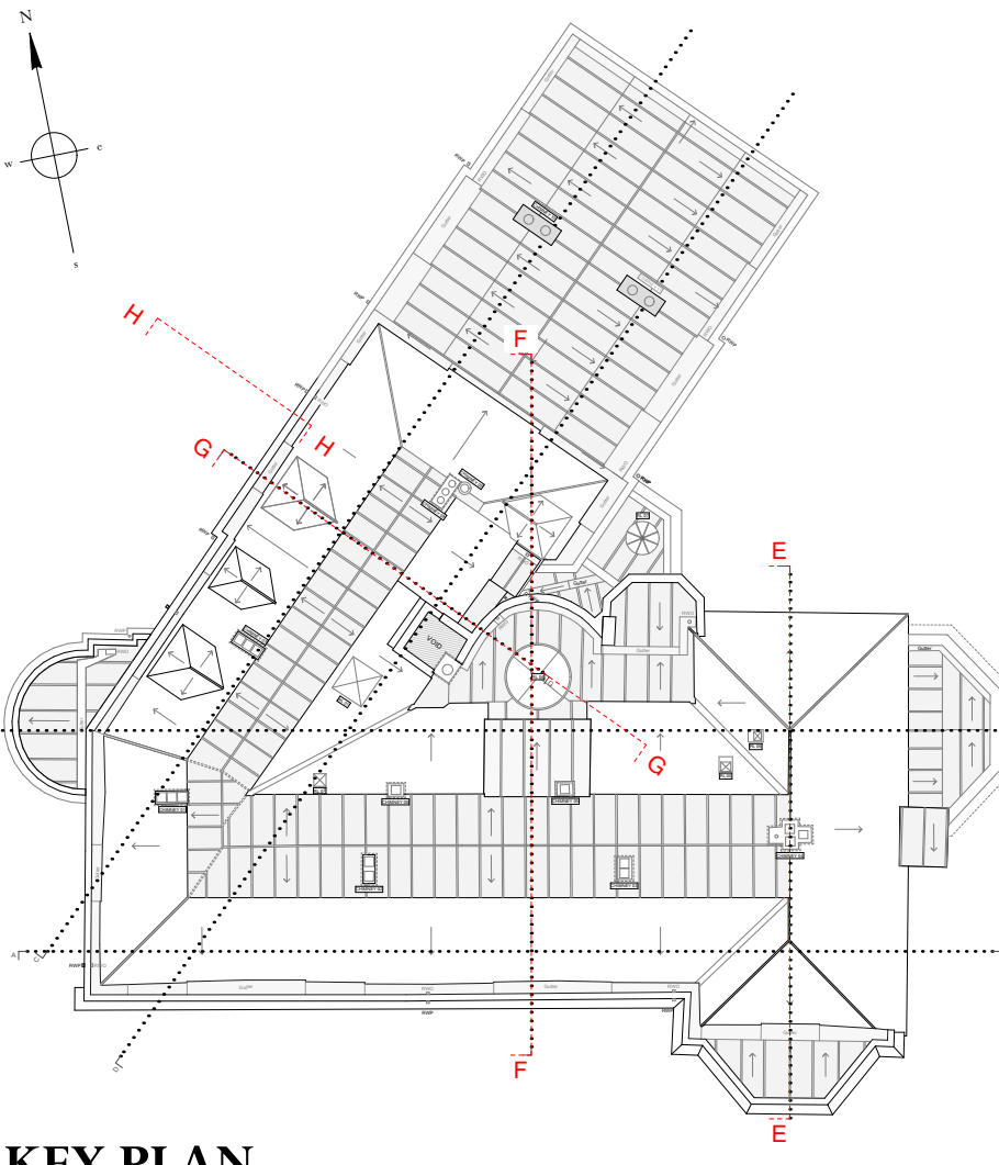
KEY PLAN
