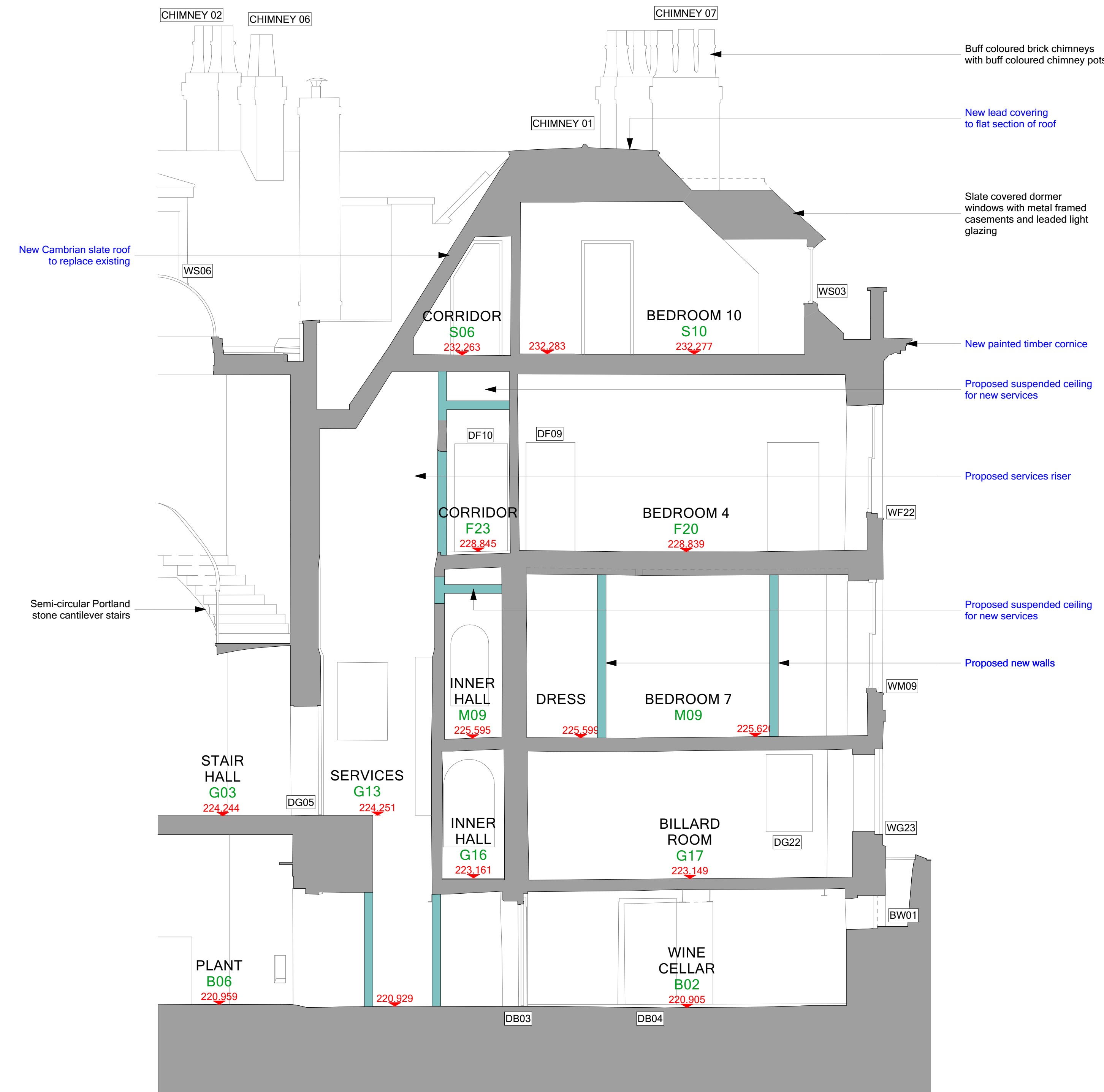
SECTION G-G
