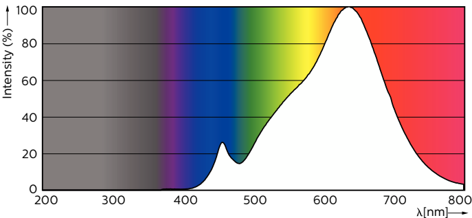
Spectral Power Distribution Colour - MASLED ExpertColor5.5-50W GU10 927 36DUK
