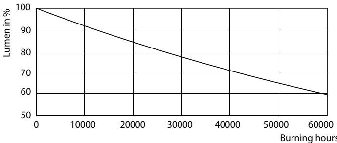
Lumen Maintenance Diagram - MASLED ExpertColor5.5-50W GU10 927 36DUK
