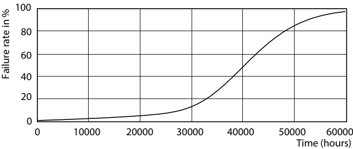
Life Expectancy Diagram - MASLED ExpertColor5.5-50W GU10 927 36DUK
