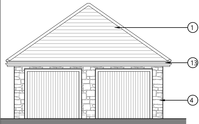
Front Elevation
