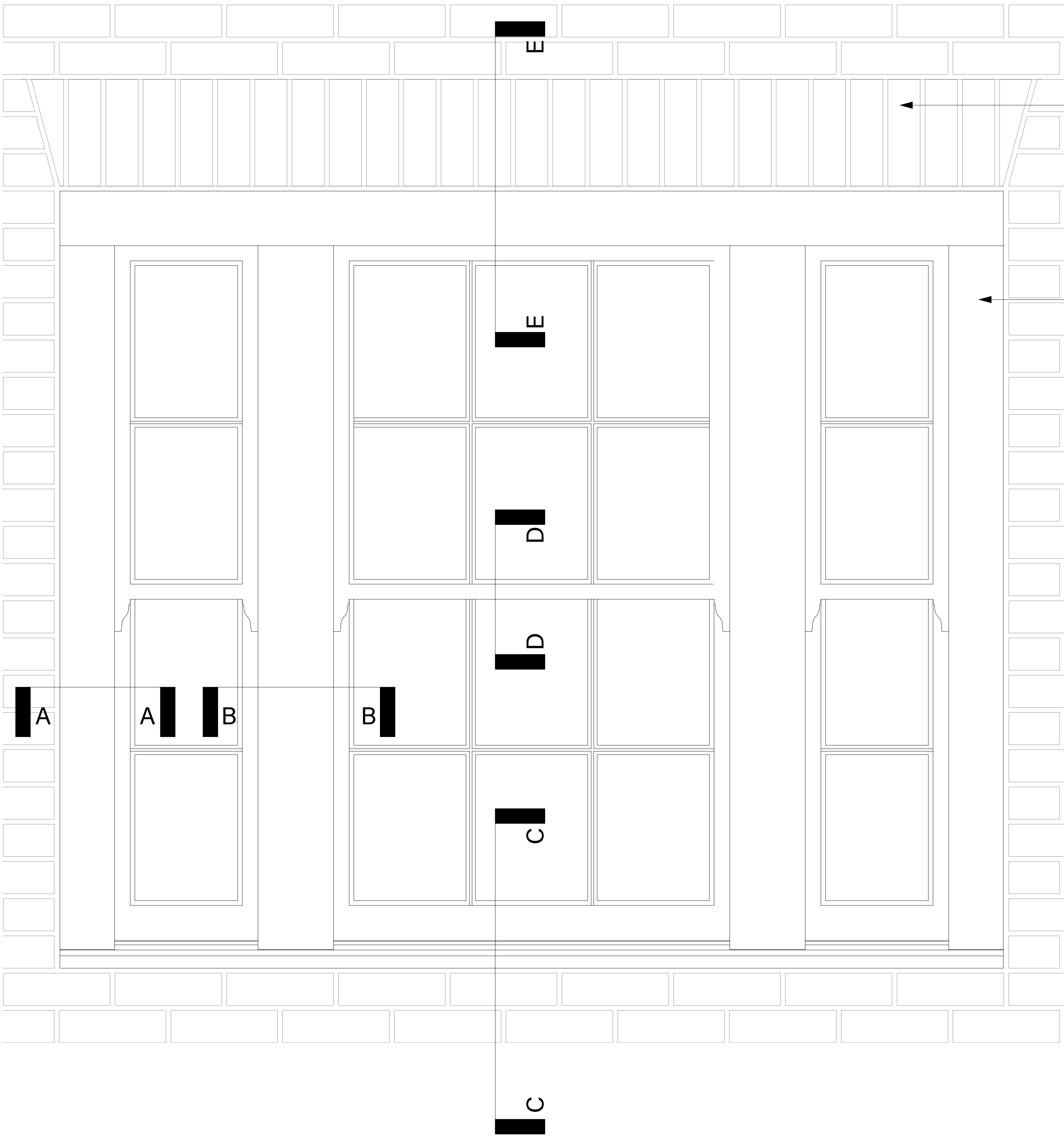
TYPICAL TIMBER SASH WINDOW ELEVATION (FALCON HOUSE) scale 1:5
