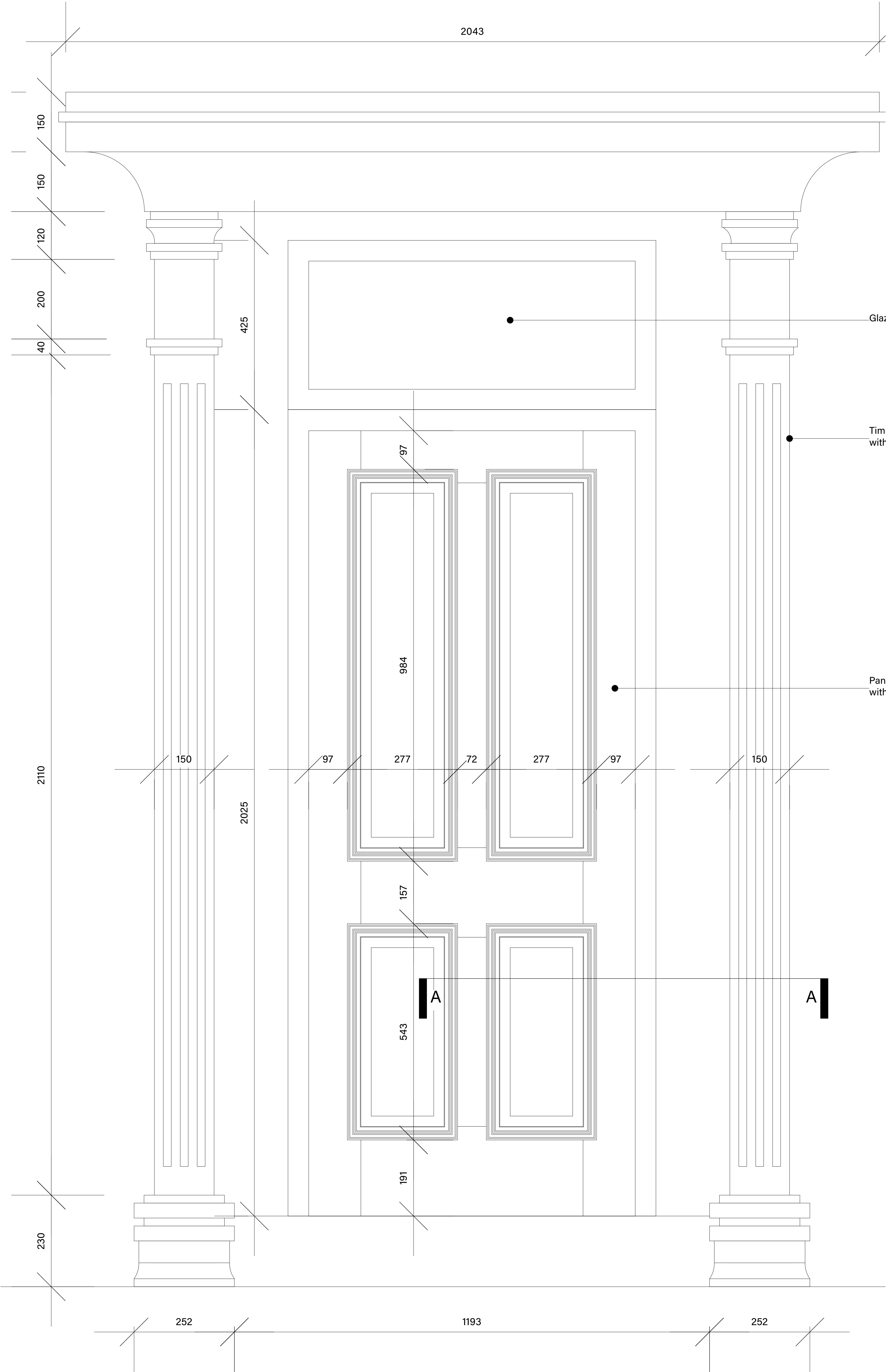
ELEVATION scale 1:5
