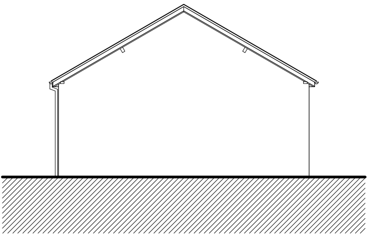
East Elevation
