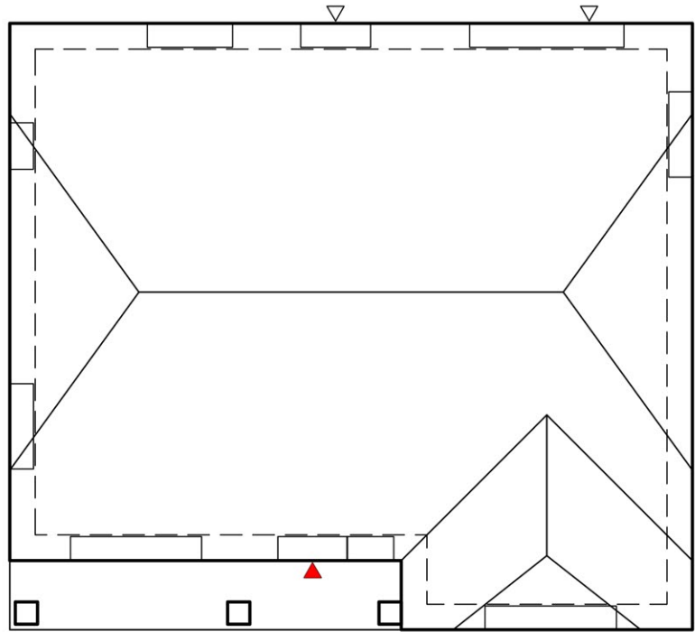
Roof Plan
